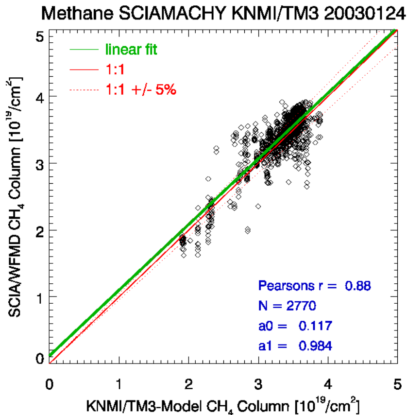
Fig. 15. Correlation of the SCIAMACHY CH 4 column measurements shown in Fig. 8 with the corresponding KNMI/TM3 model data shown in Fig. 9. The comparison is limited to measurements over land. The linear correlation coefficient r is 0.88. The number of data points N is 2770. The offset and slope parameters of the linear fit are a_0=0.12 and a_1=0.98 .
