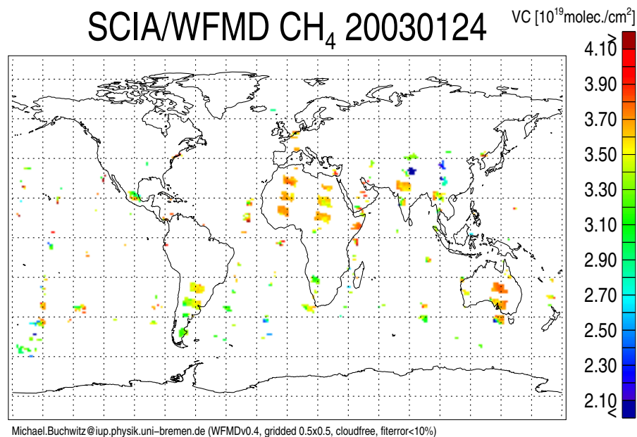
Fig. 8. As Fig. 7 but only for strictly cloud free pixels.
