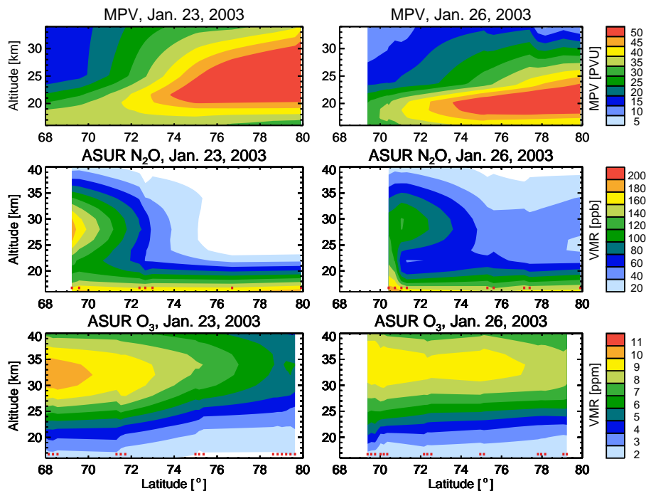
Fig. 2. Left: Modified PV from ECMWF analyses along the line of sight of the ASUR instrument (top), ASUR measurements of \text{N}_2\text{O} (middle), and ASUR ozone measurements (bottom) during the flight on 23 January 2003 on the flight leg from Spitsbergen to Kiruna. Right: ECMWF MPV, ASUR \text{N}_2\text{O} , and ASUR ozone during the flight on 26 January 2003. The small red tick marks on the bottom of the measurement contour plots indicate the position of the individual measurements.
