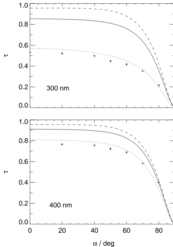
Fig. 6. Angle of incidence dependencies of FEP transmissions \tau_h (full lines) and \tau_d (dotted lines) according to Eq. (21) for a 250 \mu\text{m} FEP film. Upper panel: \lambda=300 nm, lower panel: \lambda=400 nm. Crosses indicate experimental data for the FEP material used in the construction of SAPHIR. The dashed line shows \tau_F for comparison (no bulk effects, see text).
