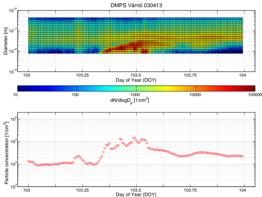
Fig. 6. Diurnal variation of Värriö size distribution and total number concentration.
