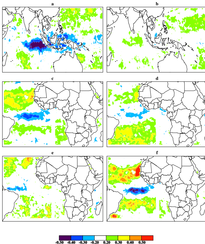
Fig. 4. Spatial correlation between anomalies monthly mean AVHRR AOT and anomalies monthly mean ISCCP total cloud amounts in biomass burning and non-biomass burning seasons in (a)–(b) : Malaysia & Indonesia; (c)–(d) : North Africa; (e)–(f) : South America and South Africa regions, the correlations are significant at the 95% level at \pm 0.2 , and >99.9% level at \pm 0.30 .
