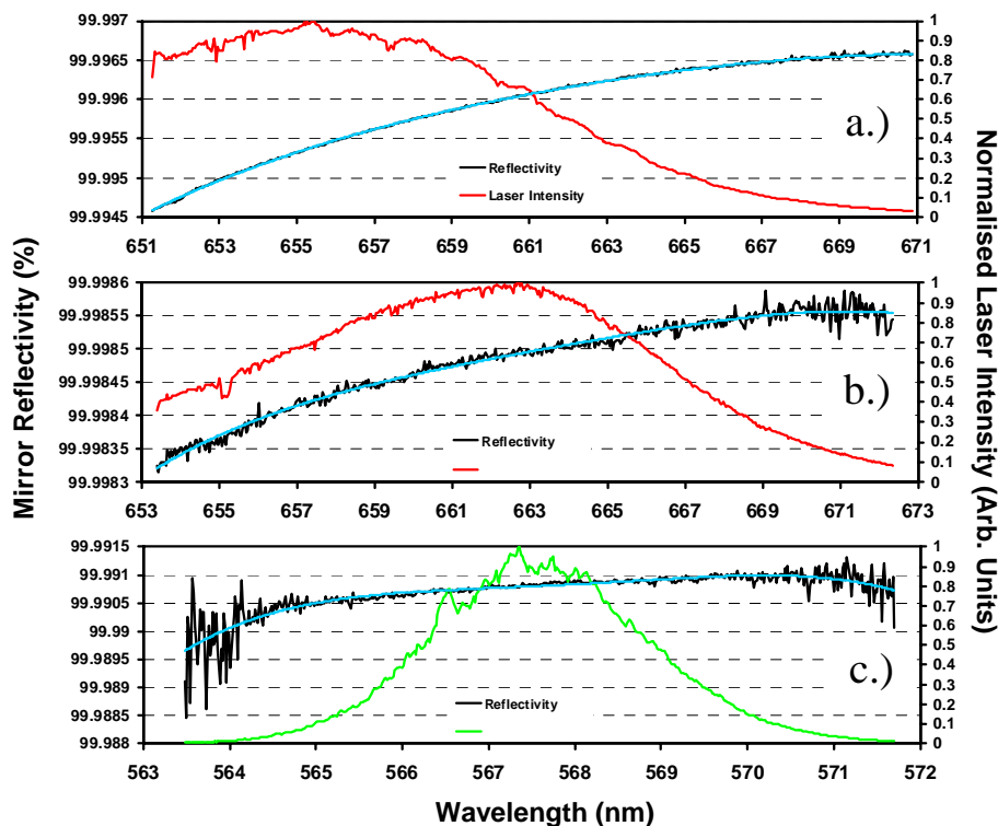
Fig. 3. Examples of the spectral distribution of the broadband dye laser output at wavelengths used to detect \text{NO}_3 and \text{N}_2\text{O}_5 (red curves) or \text{OIO} and \text{I}_2 (green curve). Panels (a) to (c) also show the wavelength dependent reflectivities of the three pairs of CRDS mirrors used during NAMBLEX (measured reflectivities in black and polynomial fits in blue; see also Table 1.)
