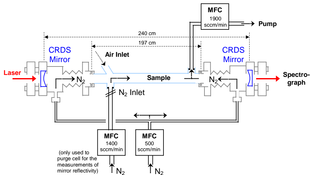
Fig. 5. The ringdown cavity and associated gas flows in the configuration used to detect \text{NO}_3 + \text{N}_2\text{O}_5 . The heated glass tube between the mirror mounts (shown in light blue) could be flushed with dry nitrogen to record the ringdown times of the empty cavity, or be removed to allow measurements of \text{NO}_3 , \text{OIO} and \text{I}_2 in an open path configuration (MFC = mass flow controller).
