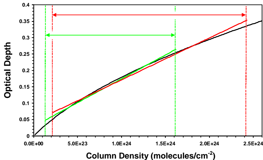
Fig. 11. The non-linear variation in the optical depth with water column amount at the resolution of the BCRDS instrument. These data are for a single wavelength on resonance with a water absorption line. The green and red lines illustrate examples of fits to retrieve the linearized absorption cross sections for ringdown decays sampling different ranges of water columns, either due to an increase in ambient [H 2 O] or to the use of a slower CCD clocking rate (green → red).
