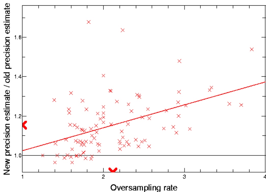
Fig. 8. The ratio “new precision estimate/old precision estimate” versus the oversampling rate (= the average number of matches to which an ozone measurement contributes). A regression line and the horizontal line corresponding to a ratio of 1 (new error bars = old error bars) have been added. Moreover, the mean values of the abscissae and the ordinates of the data points have been highlighted by triangular arrowheads. The same data as in Fig. 7 have been used.
