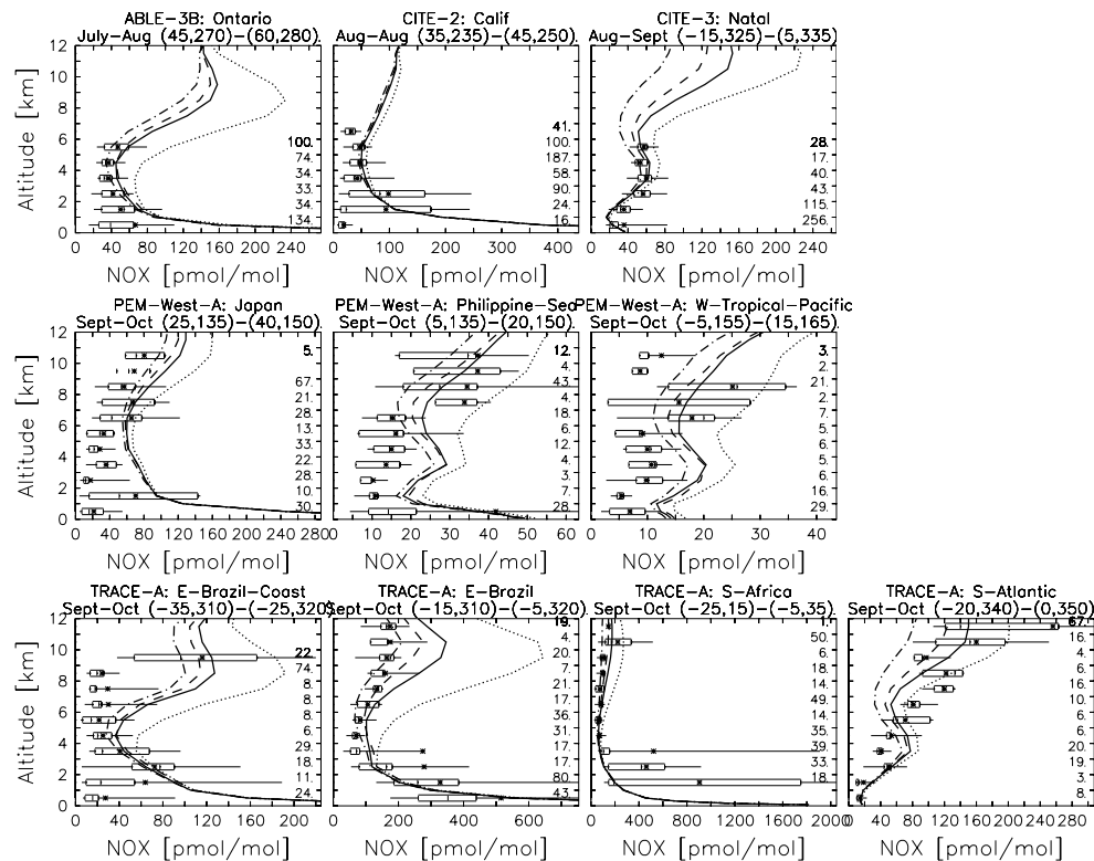
Fig. 12. NO x profiles for different campaign regions and for NoLtNO x (dash-dotted line), EVEN5(dashed line), PICK5(solid line) and PICK20 (dotted line) runs. The boxes and whiskers contain the central and side 40% of the observations. On the right-hand side are the number of observations at each altitude. Inside the whisker boxes, the median and mean values are represented by an asterisk and vertical line, respectively.
