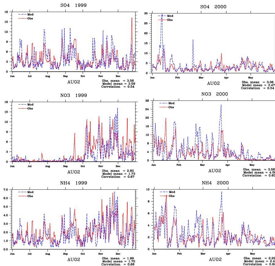
Fig. A2. Comparison of model calculated daily concentrations of secondary inorganic aerosols with observations at AU02 (Streithofen) for the period 1 June 1999–31 May 2000. Units: \mu\text{g}/\text{m}^3 .
