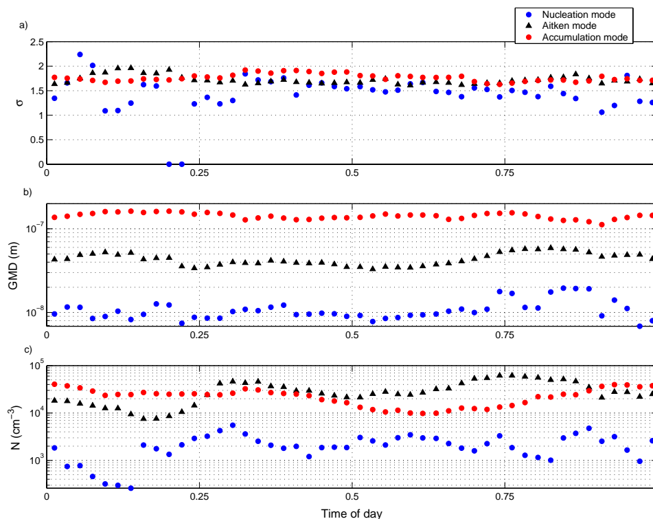
Fig. 4. Calculated geometrical mean (30 min) of the diurnal variations of modal parameters for each mode. (a) represents the geometrical standard deviation ( \sigma ), (b) the geometric mean diameter (GMD) and the (c) the aerosol particle number concentration in mode.
