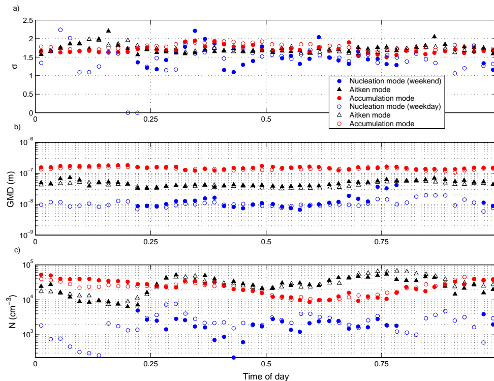
Fig. 5. Calculated geometrical mean (30 min) of the diurnal variations of modal parameters for each mode during weekends and weekdays. (a) represents the geometrical standard deviation ( \sigma ), (b) represents the geometrical mean diameter (GMD) and (c) represents the aerosol particle number concentration in mode.
