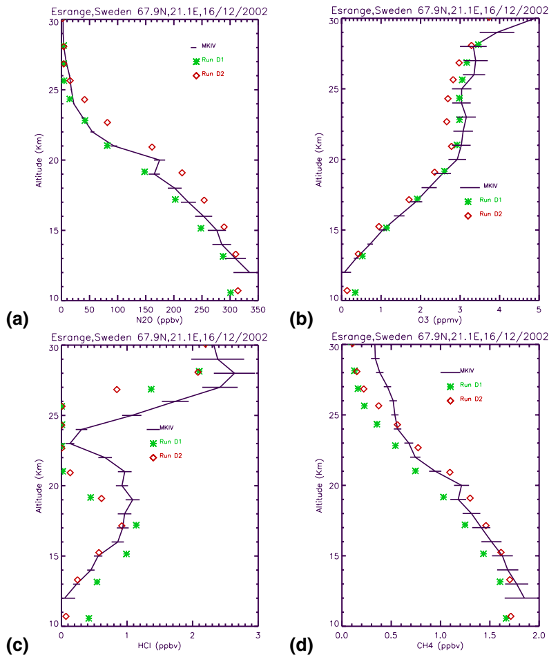
Fig. 4. MkIV balloon observations of (a) N 2 O (ppbv), (b) O 3 (ppmv), (c) HCl (ppbv) and (d) CH 4 (ppbv) at Esrange (68° N, 21° E) on 16 December 2002 along with results from SLIMCAT model runs D1 (green) and D2 (red).
