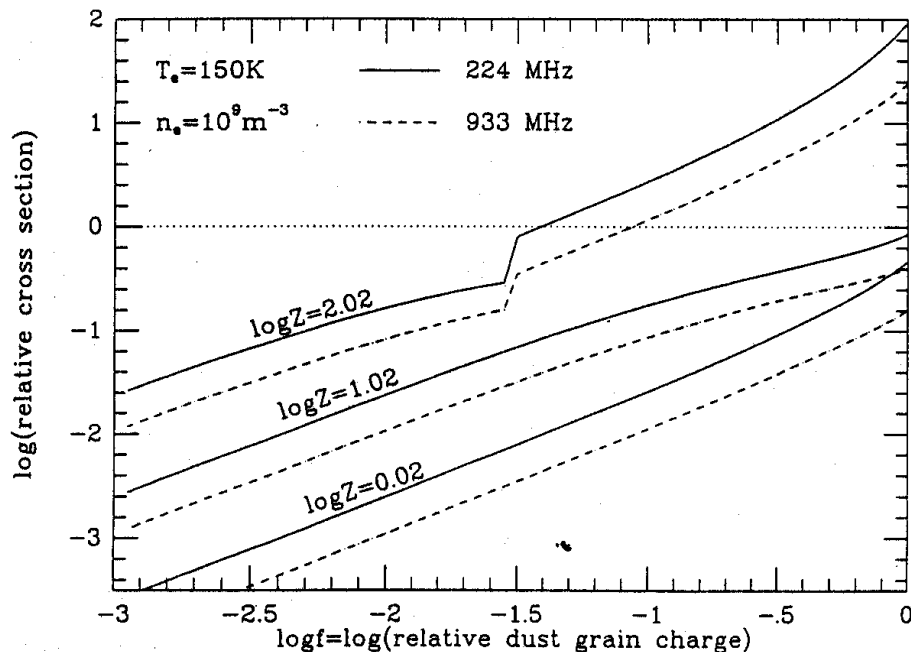
Fig. 28. Scattering cross-section of the charged dust component relative to the Thompson scattering cross section as a function of f = |Z_A|N_A/N_e , with N_e=1000 \text{ cm}^{-3} and an electron temperature T_e=150 \text{ K} for three values of the dust charge ( Z_A=Z=1 \text{ } 10 \text{ } 100 ) for the radar frequencies 224 MHz and 933 MHz (Hagfors, 1992).
