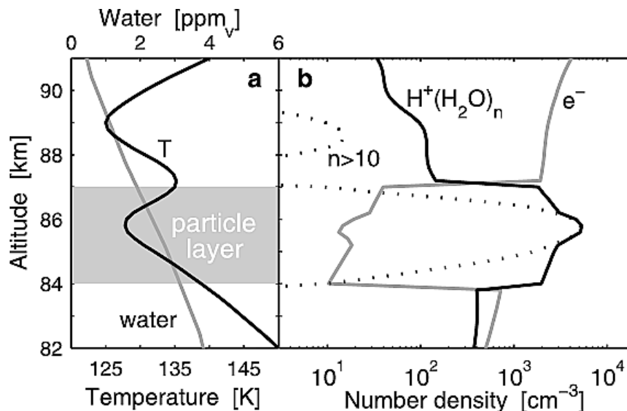
Fig. 29. (a) Input temperature and water vapor mixing ratio profiles for the model simulations by Gumbel and Witt (2002). The grey shaded area indicates the altitude range of an ice particle layer with 10^4 \text{ cm}^{-3} particles of radius 5 nm. (b) Resulting profiles of electron number density and total proton hydrate density. The dashed line denotes the contribution of larger proton hydrates (i.e. with more than 10 H_2O -ligands). This figure is reproduced from Gumbel and Witt (2002), copyright by the American Geophysical Union.
