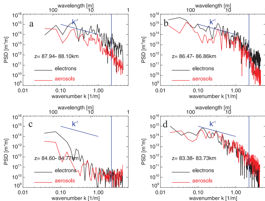
Fig. 34. Power spectra of electron number density (black lines) and particle charge number density fluctuations (red lines) shown in Figs. 32. The inclined line represents a spectral slope of -1 and the vertical line marks the radar Bragg scale ( =2.8 m) (Rapp et al., 2003a).
