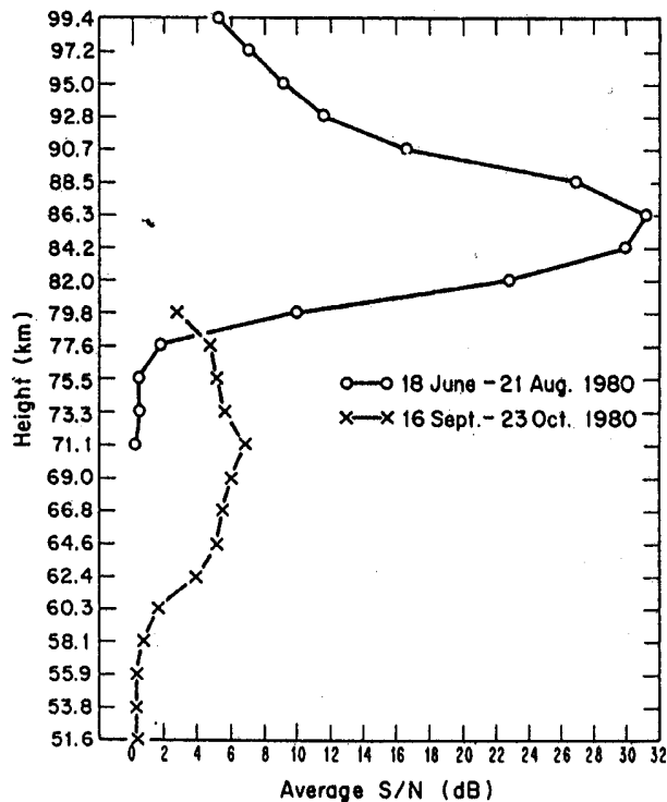
Fig. 2. Time averaged profiles of signal to noise ratio (in decibels) for typical summer and winter periods. This figure is reproduced from Ecklund and Balsley (1981) , copyright by the American Geophysical Union.
