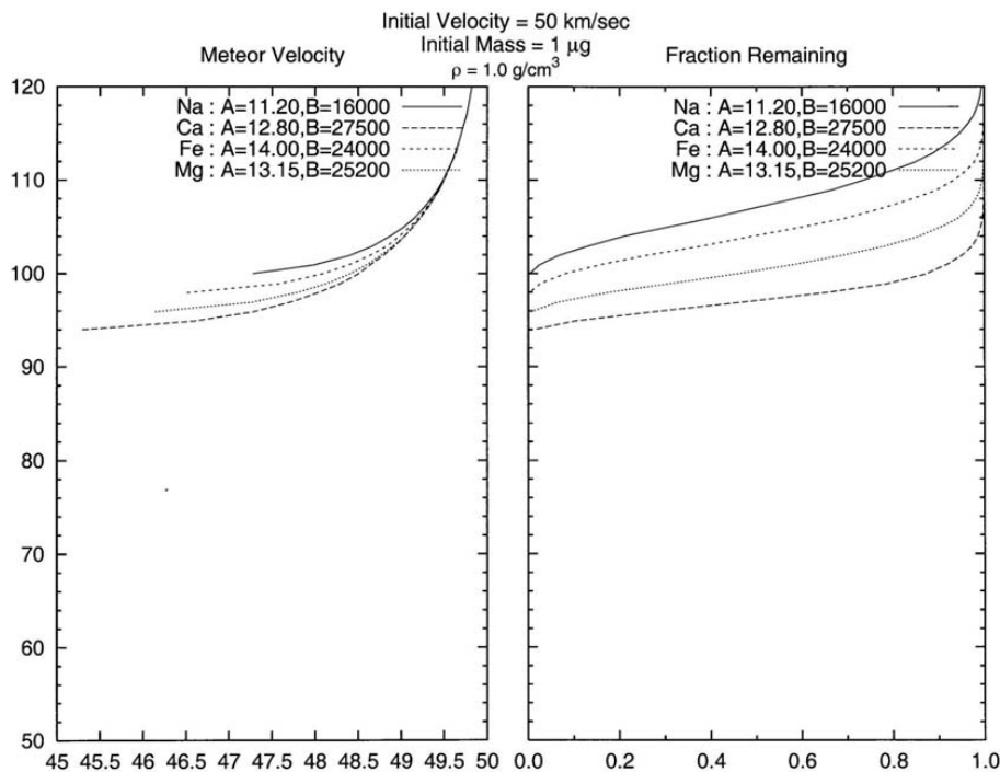
Fig. 3. The ablation of a 1 µg particle entering the atmosphere at 50 km/s.
