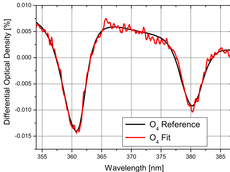
Fig. 2. Example of an \text{O}_4 fit for an elevation angle of 3^\circ on 26 April 2003. The black solid line is the scaled laboratory reference, the red line the fit result. This fit yields an \text{O}_4 DSC of 5.16 \times 10^{43} \text{ molec}^2 \text{ cm}^{-5} having a linear fit error of 0.5%. As background for this fit a zenith sky noon spectrum was used. A polynomial of degree 3, \text{NO}_2 , BrO and a modeled Ring spectrum have been included.
