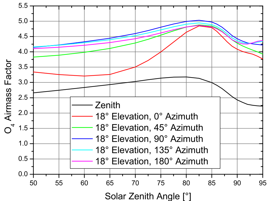
Fig. 7. Absolute airmass factors for O_4 . Pointing the instrument towards the sun ( 0^\circ relative azimuth) leads to decreasing differences between horizon and zenith sky AMF.
