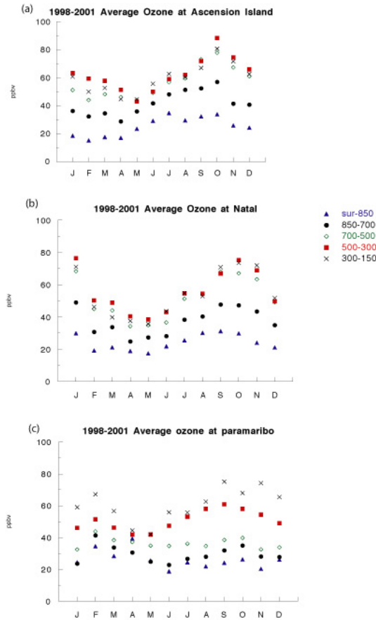
Fig. 5. 1998–2001 average ozone mixing ratios in various tropospheric layers. (a) Ascension Island, (b) Natal, (c) Paramaribo. Units are ppbv.
