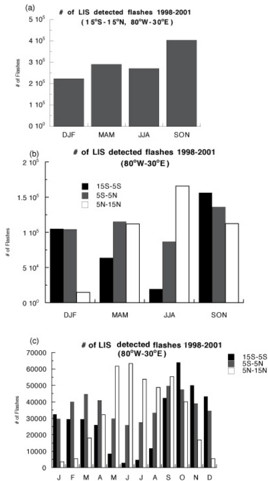
Fig. 8. 1998–2001 LIS seasonal lightning statistics: (a) total number of seasonal flashes (b) distribution of seasonal flashes for latitude zones of 15° S–5° S, 5° S–5° N, 5° N–15° N, (c) distribution of monthly flashes for latitude zones of 15° S–5° S, 5° S–5° N, 5° N–15° N.
