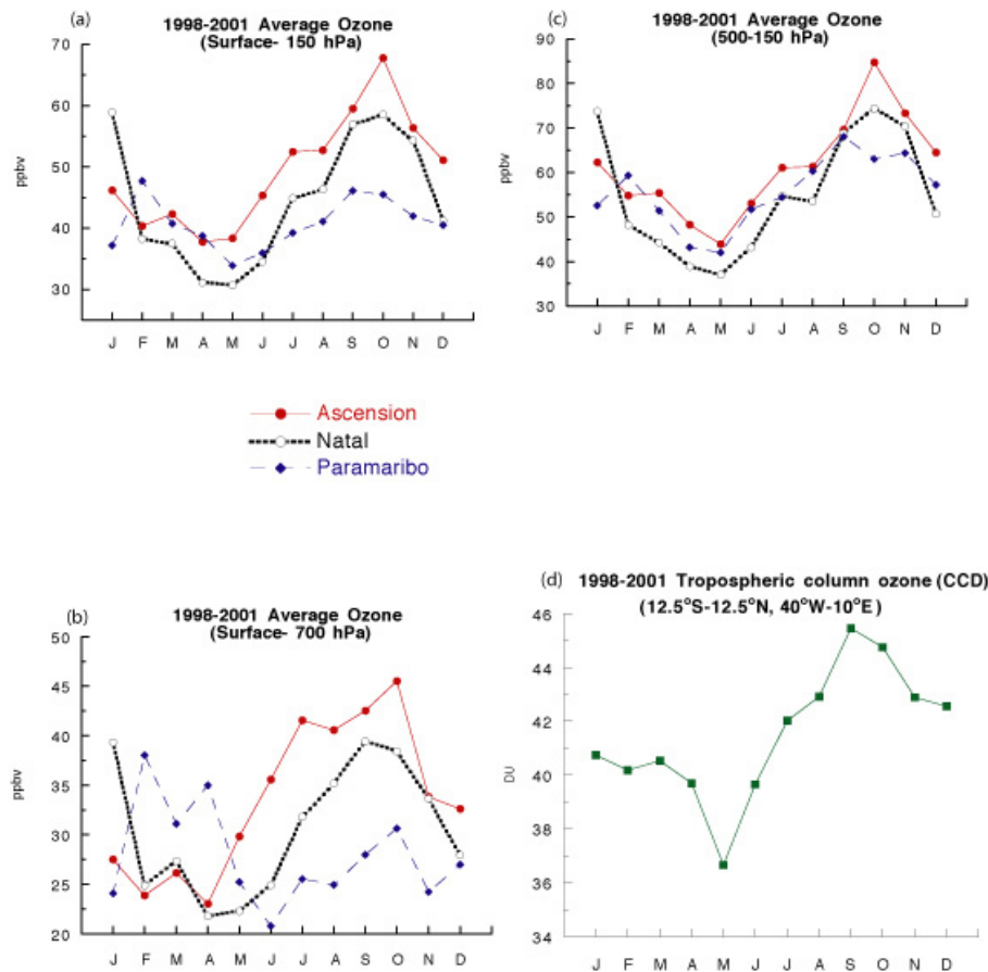
Fig. 6. 1998–2001 average ozone mixing ratios (ppbv) at Ascension Island, Natal and Paramaribo from (a) surface to 150 hPa, (b) Surface to 700 hPa, (c) 500 to 150 hPa. (d) 1998–2001 CCD tropospheric column ozone for 12.5° S–12.5° N, 40° W–10° E.
