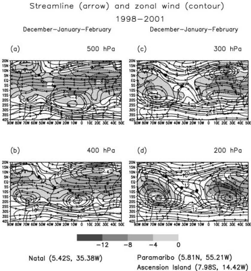
Fig. 10. 1998–2001 DJF middle/upper troposphere zonal winds and streamlines for (a) 500 hPa, (b) 400 hPa, (c) 300 hPa, (d) 200 hPa. Shaded regions are easterly winds. Units are \text{m}\cdot\text{s}^{-1} .
