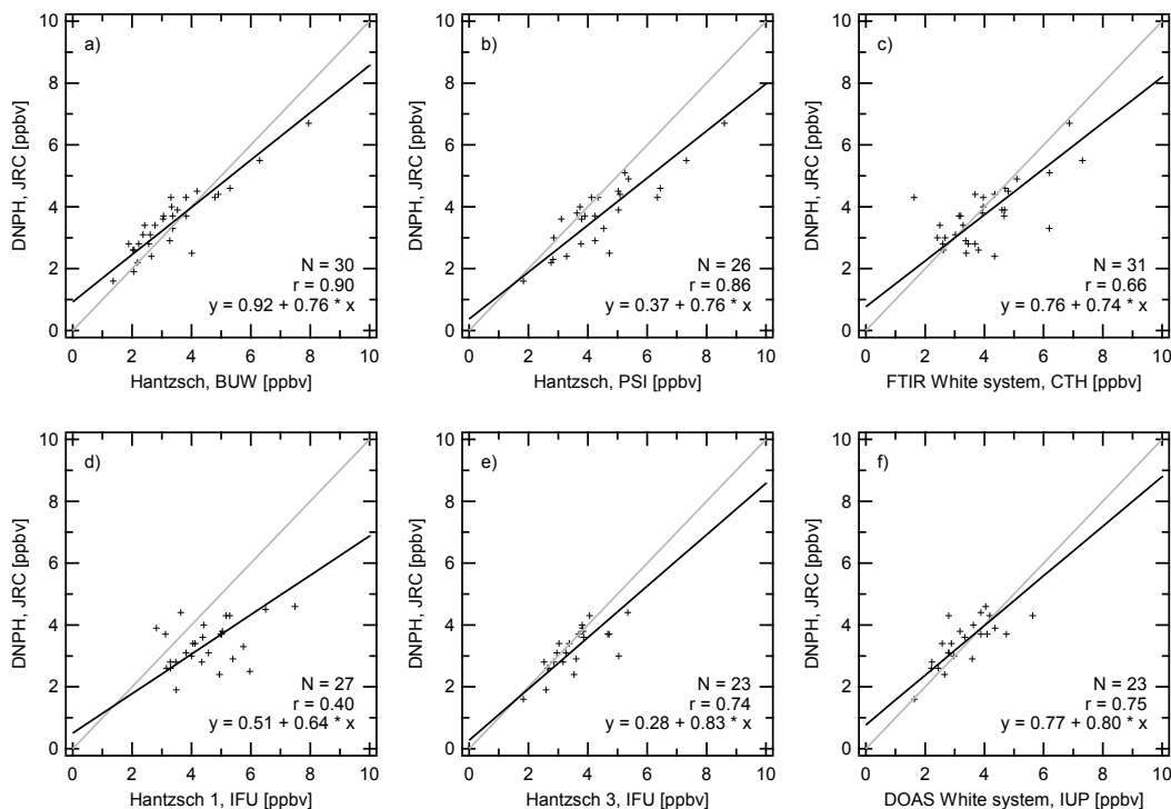
Fig. 4. Regressions of the DNPH cartridge results from the intercomparison week plotted versus those from continuous techniques for concordant two hour time spans. The solid black line drawn through the data is the orthogonal least squares fit to the data (York, 1966). The grey line represents the one to one correspondence.
