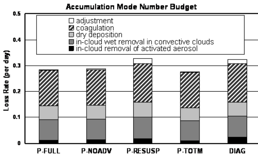
Fig. 4. Global loss budget for accumulation mode number for each treatment of cloud-borne particles. Below-cloud scavenging is negligible and hence is not plotted.
