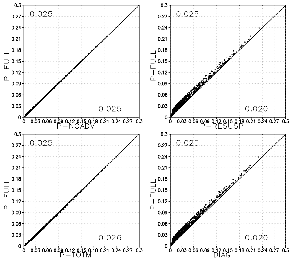
Fig. 5. As in Fig. 2, but for column accumulation mode mass.
