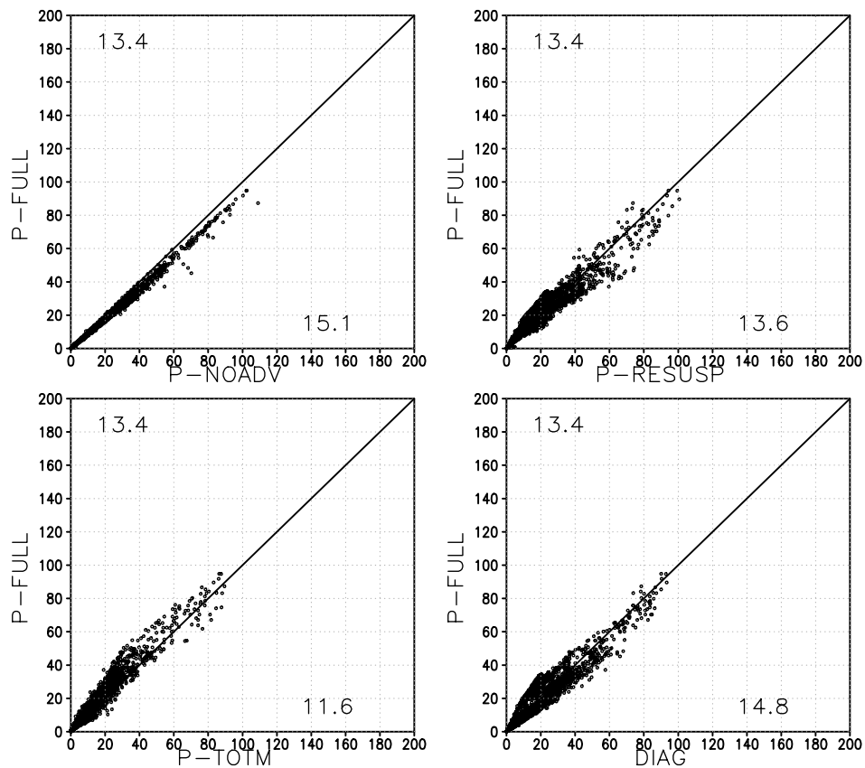
Fig. 6. As in Fig. 2, but for column cloud-borne accumulation mode number.
