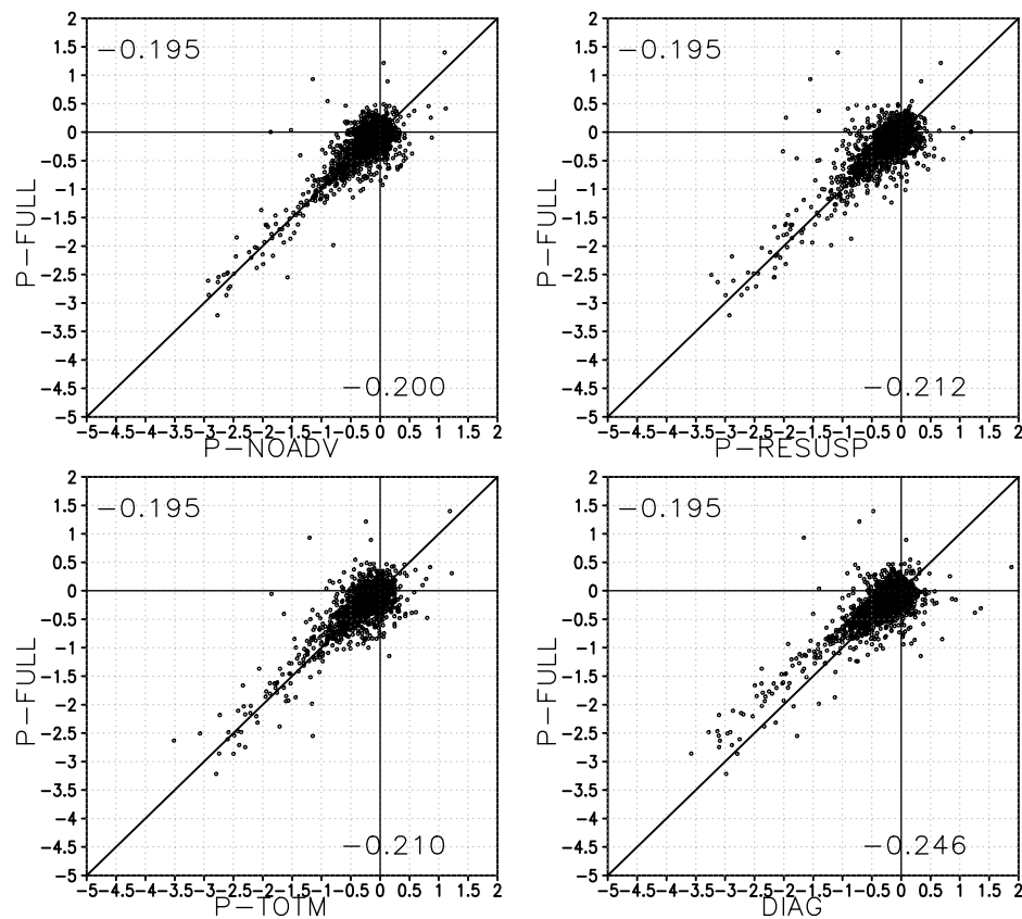
Fig. 10. As in Fig. 2, but for indirect effect due to anthropogenic sulfur.
