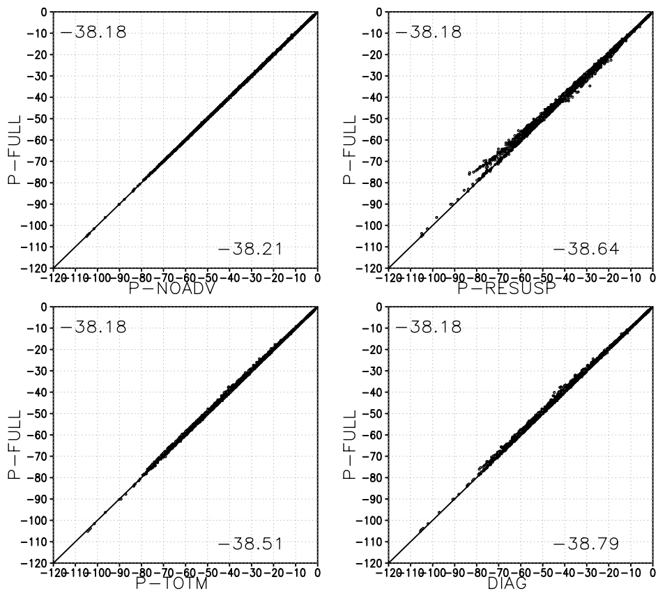
Fig. 9. As in Fig. 2, but for shortwave cloud radiative forcing.
