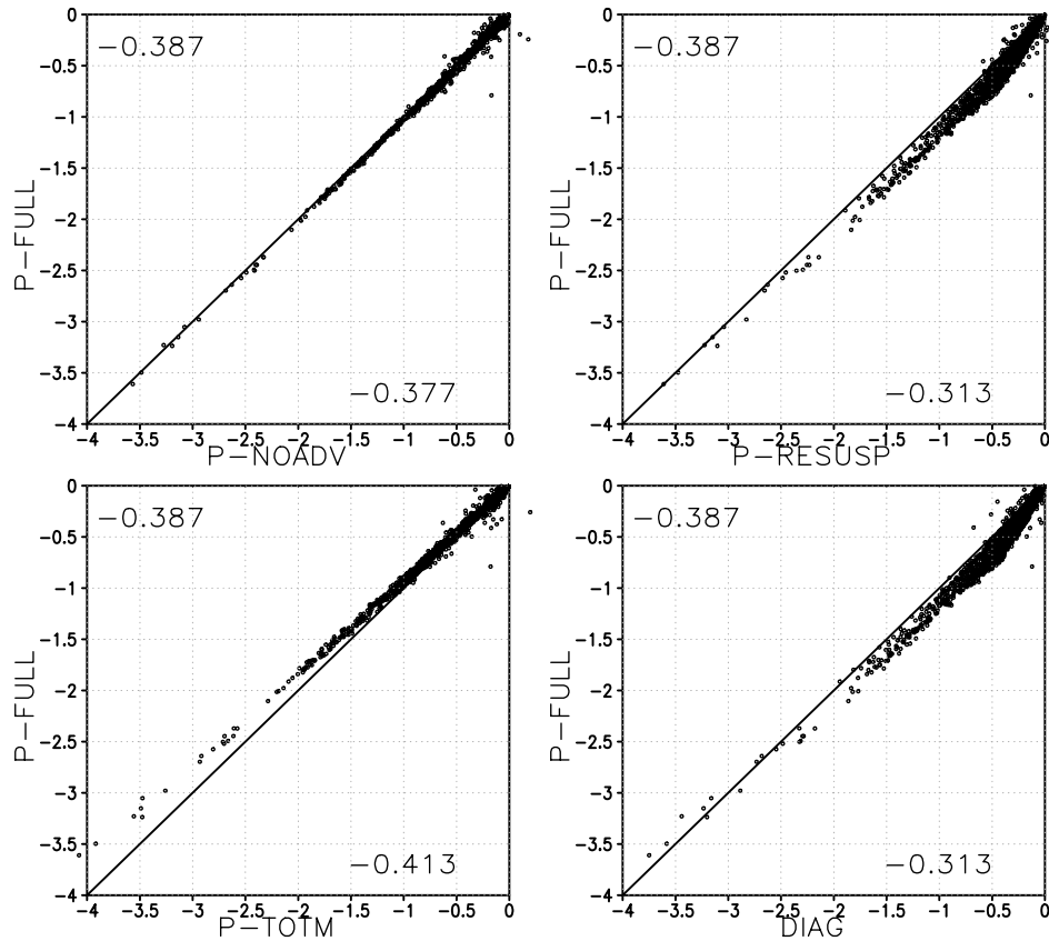
Fig. 13. As in Fig. 2, but for direct forcing due to anthropogenic sulfur.
