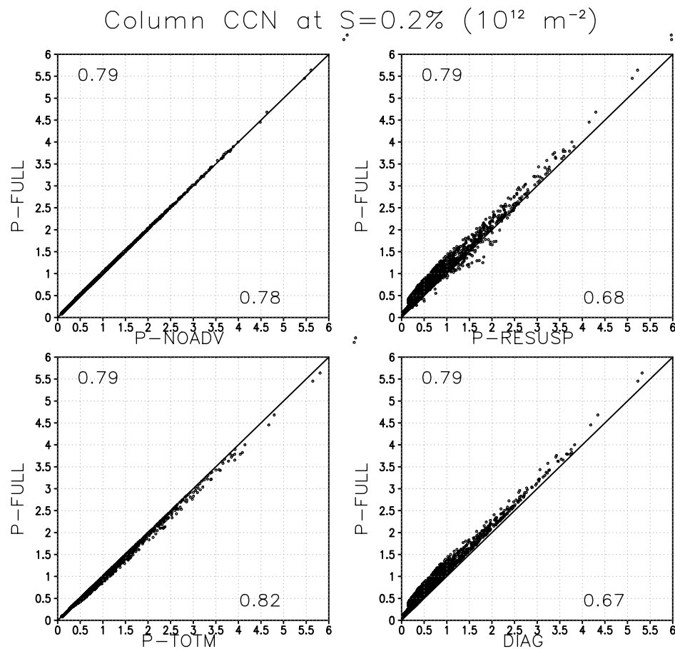
Fig. 8. As in Fig. 2, but for CCN concentration at a supersaturation of 0.2%.
