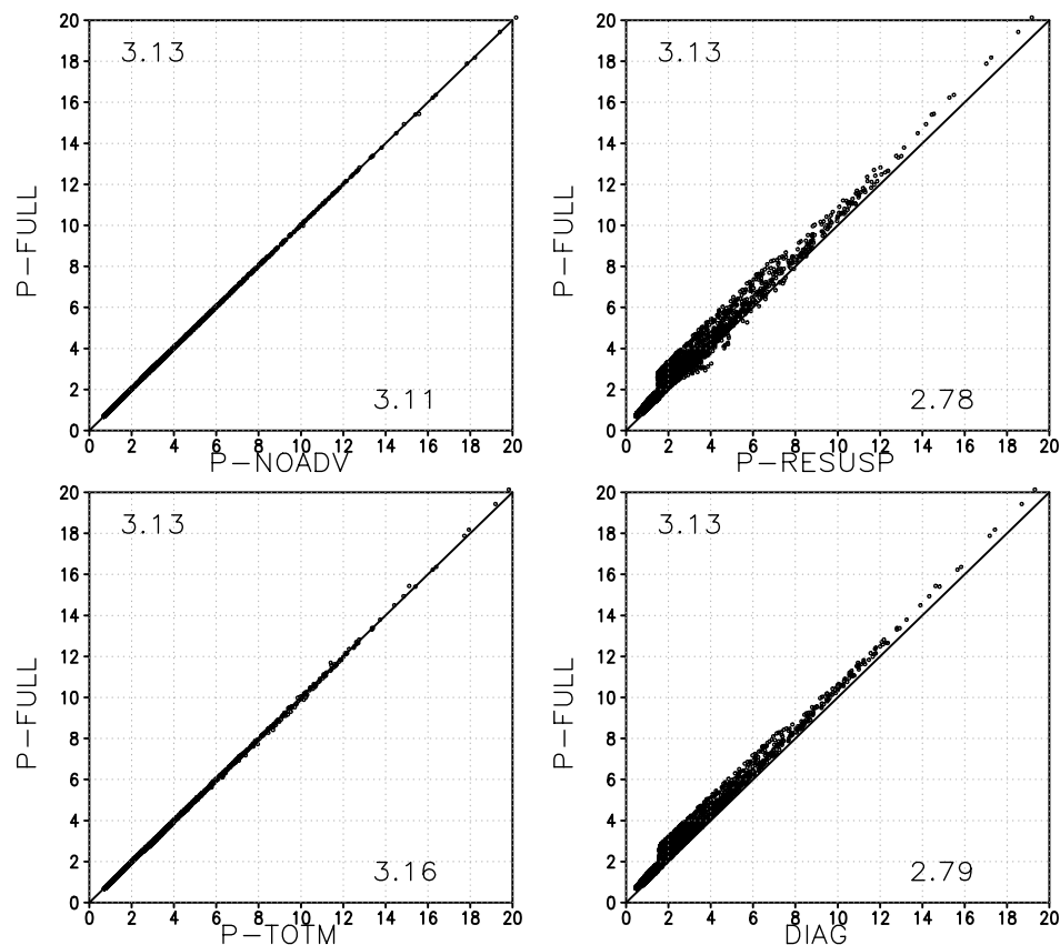
Fig. 2. Scatterplots of annual mean column integrated accumulation mode particle number concentration (cloud-borne + interstitial) for the reference treatment vs. each of the four approximate treatments. The global means for the reference and other treatments are printed in the upper-left and lower-right corners of each plot, respectively.
