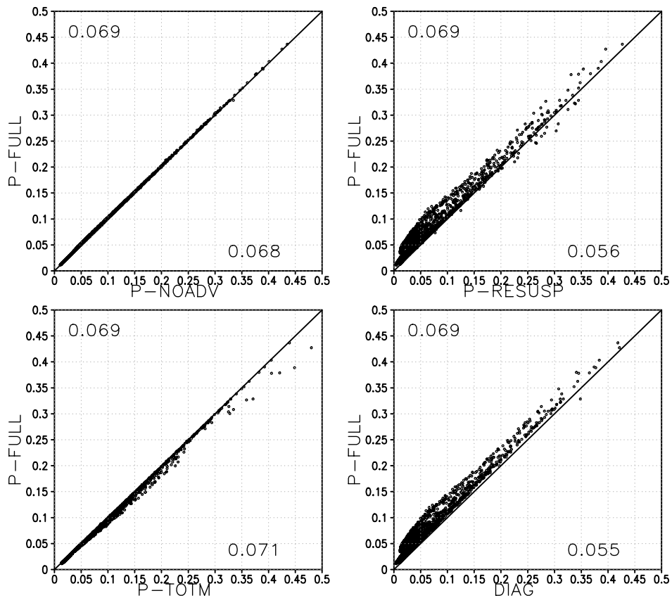
Fig. 11. As in Fig. 2, but for accumulation mode aerosol optical depth.
