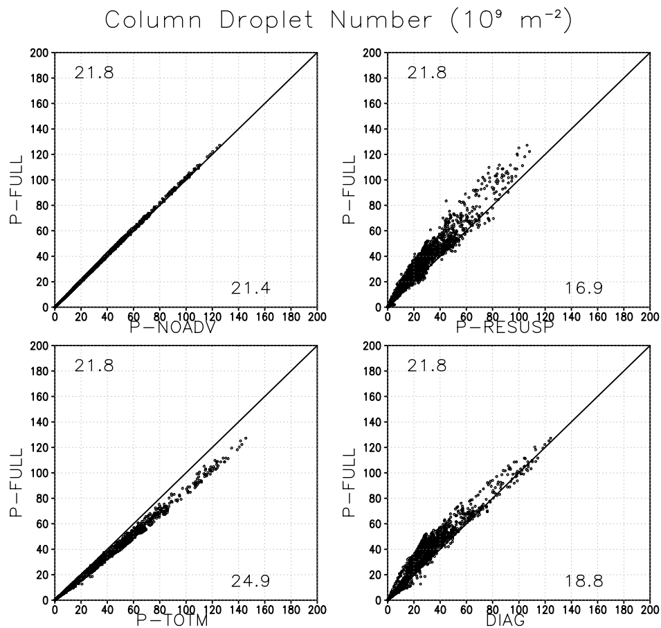
Fig. 7. As in Fig. 2, but for column stratiform-cloud droplet number.
