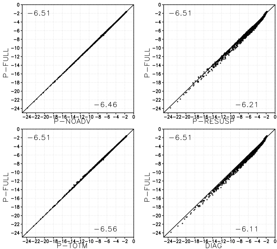
Fig. 12. As in Fig. 2, but for direct forcing by total aerosol.
