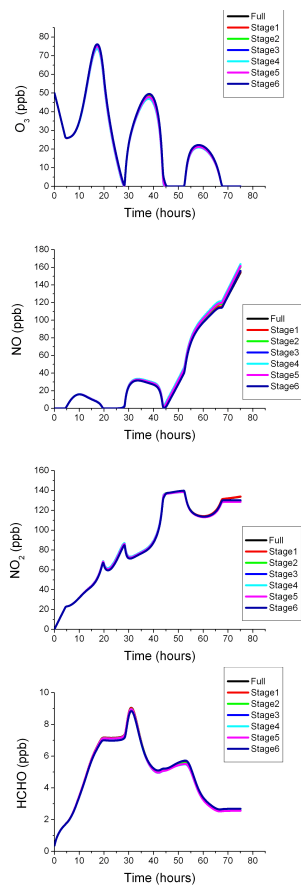
Fig. 3. Plot of trajectory 7 to stage 6 for \text{O}_3 , \text{NO} , \text{NO}_2 , \text{HCHO} .
