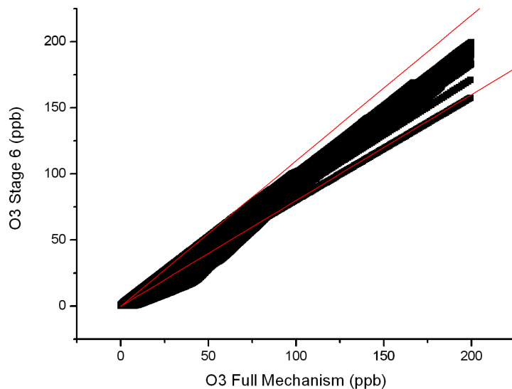
Fig. 9. Figure demonstrating the relationship between the ozone in the full mechanism and the stage 6 lumped mechanism. The upper red lines indicates a 10% variation above the full mechanism values, and the lower red line indicates a 20% variation below.
