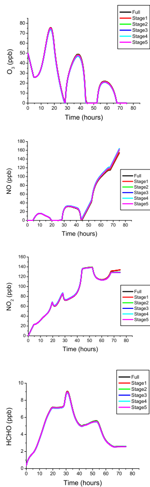
Fig. 4. Plot of Trajectory 7 to Stage 5 for O 3 , NO, NO 2 , HCHO.
