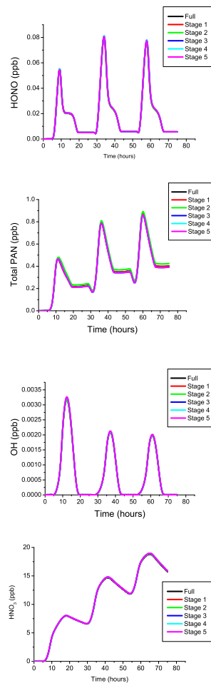
Fig. 9. Plot of Trajectory 63 to Stage 5 for HONO, total PAN, OH and HNO 3 .
