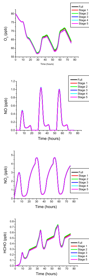
Fig. 8. Plot of Trajectory 63 to Stage 5 for O 3 , NO, NO 2 HCHO.
