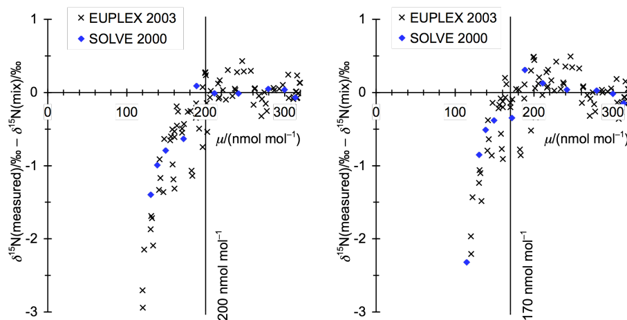
Fig. 11. Residuals of linear fits to polar aircraft N 2 O measurements. No structure is visible in the residuals for a lower cut-off of 200 nmol mol -1 (left panel), but if a lower cut-off of 170 nmol mol -1 (right panel) is used for the linear fits, samples closer to 170 nmol mol -1 fall mostly above the x-axis, while samples closer to 300 nmol mol -1 fall mostly below the x-axis.
