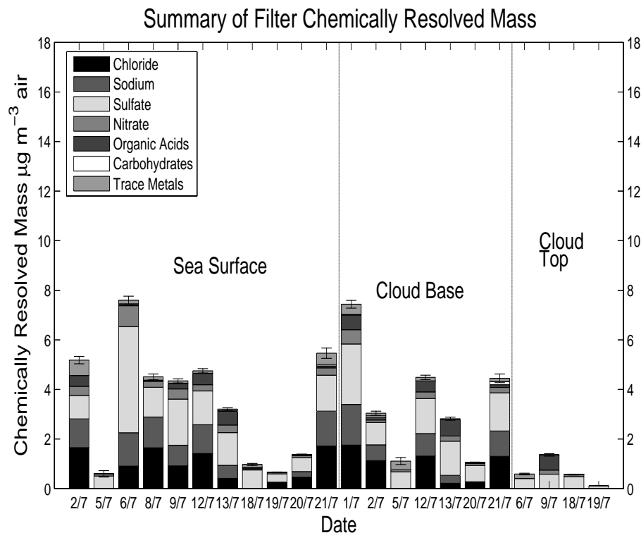
Fig. 2. Results of chemical speciation analyses of the aerosols collected aboard the Twin Otter using Teflo™ filters. Results are divided both by the day which they were collected and the level collected within the marine boundary layer.
