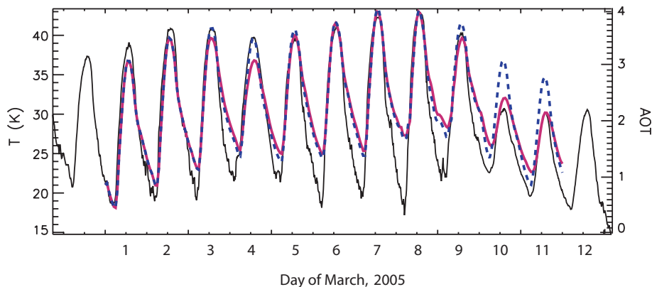
Fig. 9. 2-m Temperature difference of the regional model results including dust forcing (red line) and results from the model without including dust (blue dotted line) compared to 2 m temperature measurements at the Chicha site (black line).
