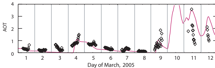
Fig. 2. Dust optical thickness computed with the box model (red line) compared to sunphotometer measurements at the Chicha site (black symbols).
