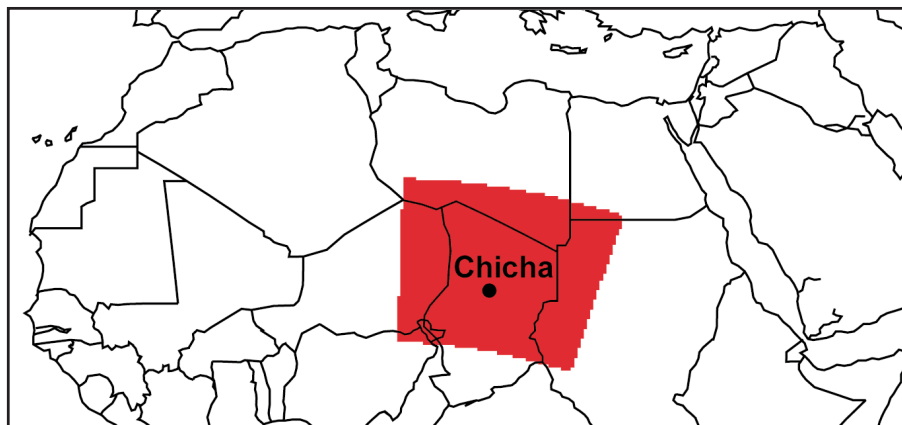
Fig. 1. Location of the field site “Chicha” in the Bodélé depression, Chad. The domain of the regional model is indicated in red.
