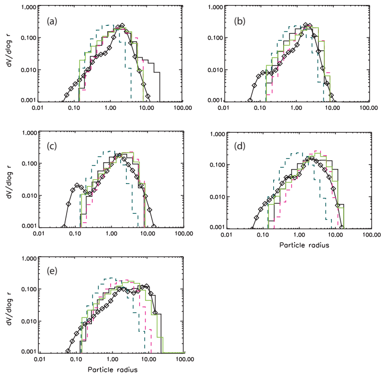
Fig. 3. Size distribution for date and times in March 2005: 4 March, 06:30 UTC (a) ; 6 March, 07:40 UTC (b) ; 7 March, 07:40 UTC (c) ; 7 March, 14:17 UTC (d) ; 9 March, 09:58 UTC (e) . Comparison of Cimel retrievals (symbols) with the size distribution from the best result from box model with (i) dust sizes modes of 1 and 10 \mu\text{m} radius and geometric standard deviation of 2, (black histograms); (ii) one dust size mode at 1 \mu\text{m} radius but with a geometric standard deviation of 3 (green histogram); (iii) as (i) but higher kinetic energy of saltating particles required for breaking up aggregates (pink dashed histogram); (iv) parameterization from Tegen et al. (2002) (blue dashes histogram).
