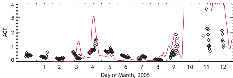
Fig. 7. Dust optical thickness computed with LM-MUSCAT (red line) compared to sunphotometer measurements at the Chicha site (black symbols).
