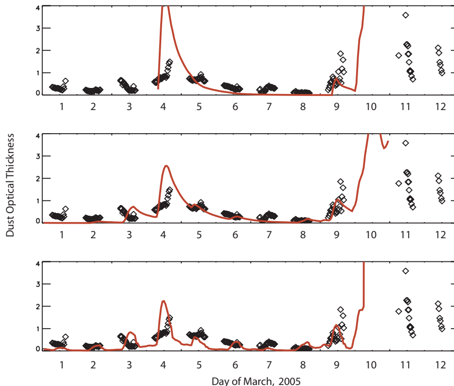
Fig. 5. Sensitivity studies of the modelled DOT (red line) at Chicha with dust emissions computed from the modelled LM surface winds and DOTs computed with the box model. Results are shown for DOT the best estimate parameter combination derived with observed winds (a); with minimum threshold wind friction velocity reduced by the factor 0.66 (b); and using a Weibull distribution to describe subgridscale variability of surface winds (c); compared to sunphotometer measurements of DOT (black symbols).
