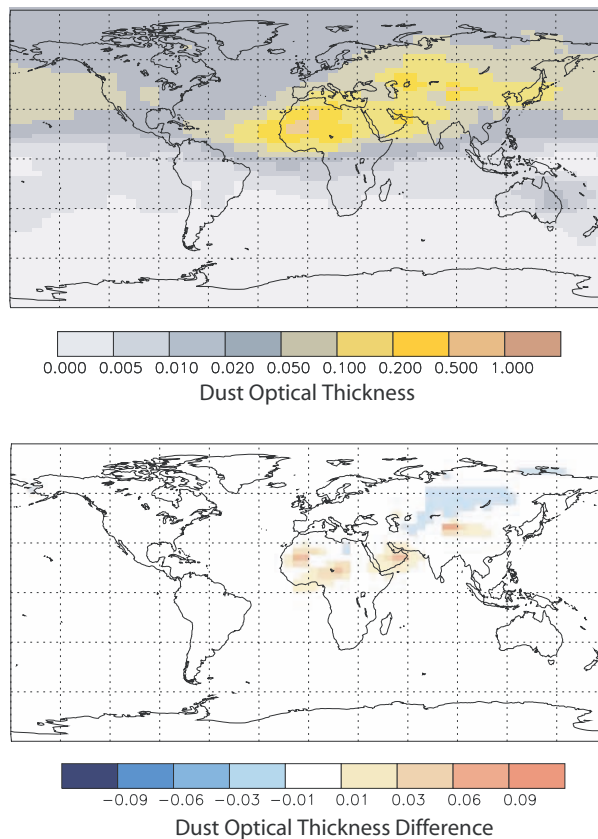
Fig. 11. Annual average modelled global dust optical thickness (top) and difference to dust optical thickness computed using the parameterization from Tegen et al. (2002) for computing dust emissions from preferential source areas (bottom) as annual mean for the example year 1987 computed with TM3/ERA15.
