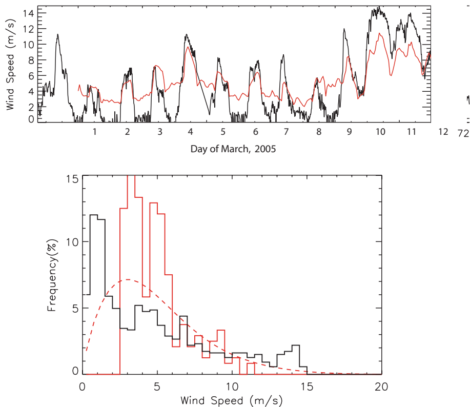
Fig. 4. Time dependent 2 m wind speed measurements (black line) compared to 10 m surface wind speed results from the LM experiment (red line; a ) and the histogram of frequencies of the wind speeds occurring in the measurements (black) and in LM (red) between days 60 to 72 ( b ). Also shown is the wind speed distribution of the model winds modified by a Weibull probability distribution (dashed red line).
