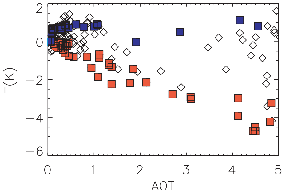
Fig. 10. Difference in modelled 2 m temperatures between the regional model experiment including dust and the modelled temperatures when dust is not included depending on dust optical thickness; the maximum day (orange) and minimum night temperatures (blue) are shown as squared symbols.
