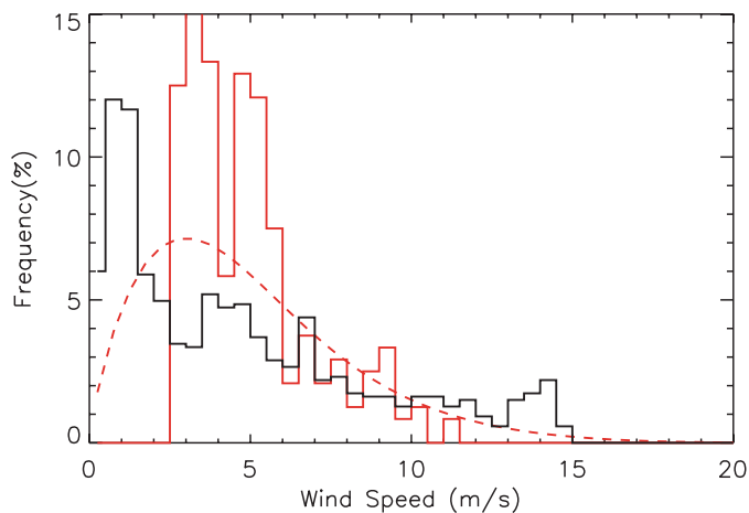
Fig. 4. Time dependent 2 m wind speed measurements (black line) compared to 10 m surface wind speed results from the LM experiment (red line; a ) and the histogram of frequencies of the wind speeds occurring in the measurements (black) and in LM (red) between days 60 to 72 ( b ). Also shown is the wind speed distribution of the model winds modified by a Weibull probability distribution (dashed red line).
