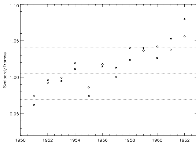
Fig. 7. Ratios of daily mean total ozone at Svalbard and Tromsø, averaged from April to July in each year (asterisks: DS+ZB; diamonds: DS+ZB+ZC). The dashed lines represent the long-term mean ( \pm 1 standard deviation) of the ratio of April-to-July averaged total ozone at Svalbard and Tromsø based on TOMS data (1979–1989).
