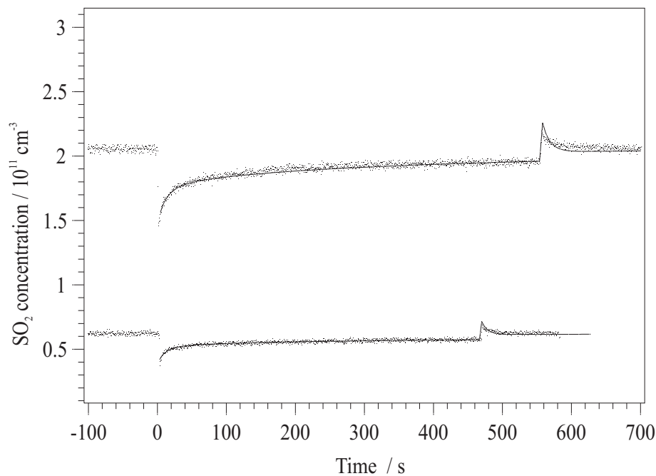
Fig. 8. Comparison of experimental (dots) and simulated (lines) data. The model parameters used are given in Table 2.
