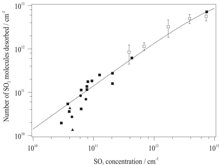
Fig. 7. Molecules of SO 2 released into the gas-phase, following exposure of a mineral dust surface, plotted as a function of initial SO 2 concentration. Squares: T=295 K, 0% relative humidity; circles: T=258 K, 0% relative humidity; triangles: T=258 K, 27% relative humidity; diamond: T=295 K, 0% relative humidity, ozone present in the carrier gas at a concentration of ~10 13 molecule cm -3 .
