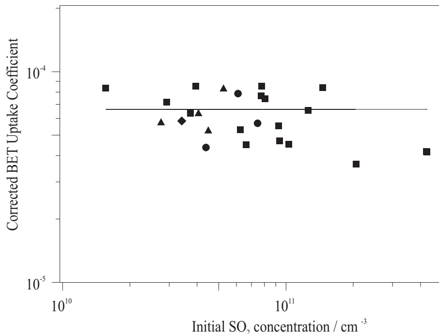
Fig. 4. Corrected initial (BET) uptake coefficients plotted as a function of initial SO 2 concentration. Squares: room temperature not humidified; circles: 258 K not humidified; triangles: 258 K, humidified; diamond: ozone present in the carrier gas at a concentration of \sim 10^{13} molecule cm -3 . The line represents the average values for unhumidified surfaces at room temperature.
