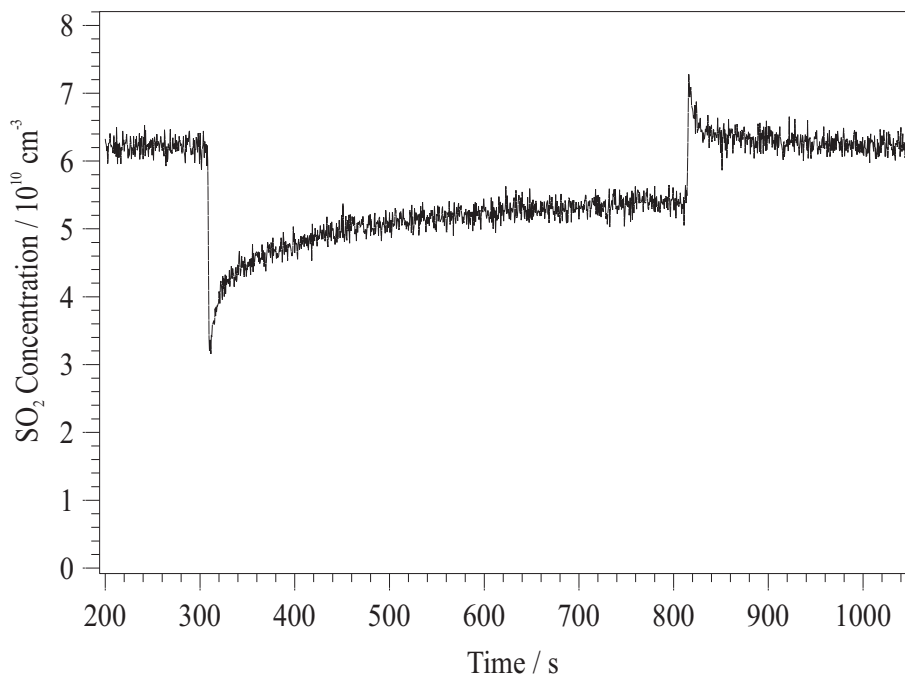
Fig. 2. Uptake of SO 2 on an unhumidified Saharan Dust surface at 295 K. The injector was withdrawn 7.4 cm at 310 s to expose ~6.7 mg of dust and returned to its original position at 820 s. Total pressure 1.5 Torr.
