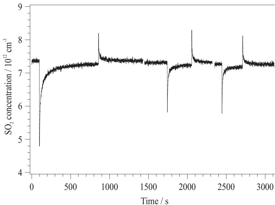
Fig. 5. Multiple uptakes onto the same dust sample. The injector was repeatedly withdrawn 6.9 cm to expose ~15 mg of dust. Total pressure 1.5 Torr.
