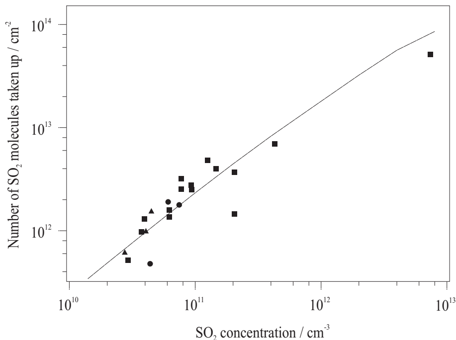
Fig. 6. Calculated surface coverage, following uptake of SO 2 onto fresh dust surfaces plotted as a function of initial SO 2 concentration. Squares: T=295 K, 0% relative humidity; circles: T=258 K, 0% relative humidity; triangles: T=258 K, 27% relative humidity; diamond: T=295 K, 0% relative humidity, ozone present in the carrier gas at a concentration of \sim 10^{13} molecule cm -3 . The line is the predicted amount of SO 2 taken up per unit area from the model described in Sect. 4.3.
