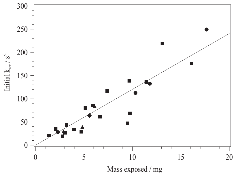
Fig. 3. Variation of the corrected initial first order loss coefficient with mineral dust mass loading. Squares: room temperature not humidified; circles: 258 K not humidified; triangles: 258 K, humidified; diamond: ozone present in the carrier gas at a concentration of \sim 10^{13} molecule \text{cm}^{-3} .
