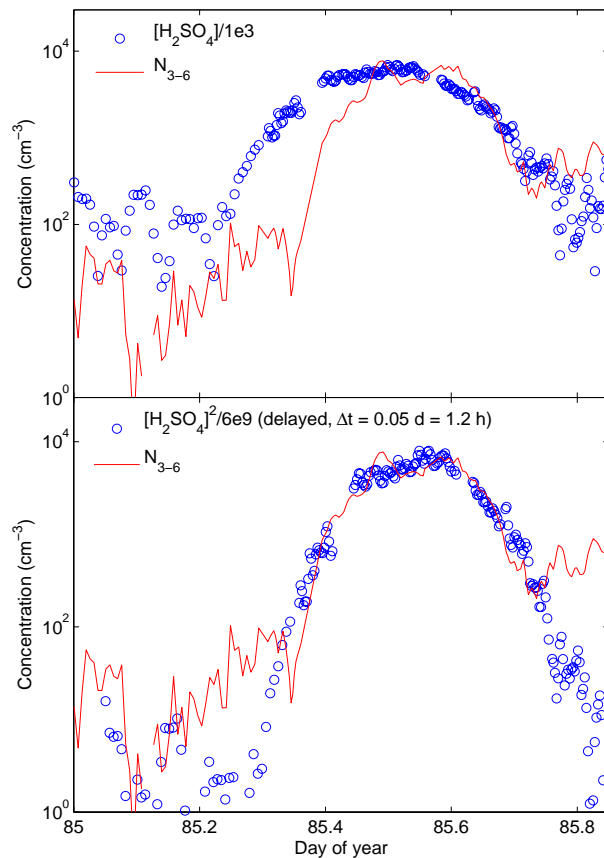
Fig. 2. (a) (upper panel) Number concentration of 3–6 nm particles ( N_{3-6} ) and sulphuric acid concentration (scaled) for day 85 (26 March 2003). (lower panel) N_{3-6} and [H_2SO_4]^2 (scaled) delayed by the time shift \Delta t = 1.2 h, showing clear correlation between N_{3-6} and [H_2SO_4]^2 during the event.
