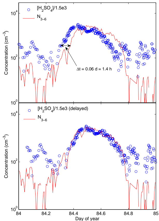
Fig. 1. (a) (upper panel) Number concentration of 3–6 nm particles ( N_{3-6} ) and sulphuric acid concentration (scaled) for day 84 (25 March 2003). The time shift \Delta t between the curves is marked by an arrow. (lower panel) N_{3-6} and [\text{H}_2\text{SO}_4] delayed by the time shift \Delta t=1.4 h, showing excellent correspondence between N_{3-6} and [\text{H}_2\text{SO}_4] during the event.
