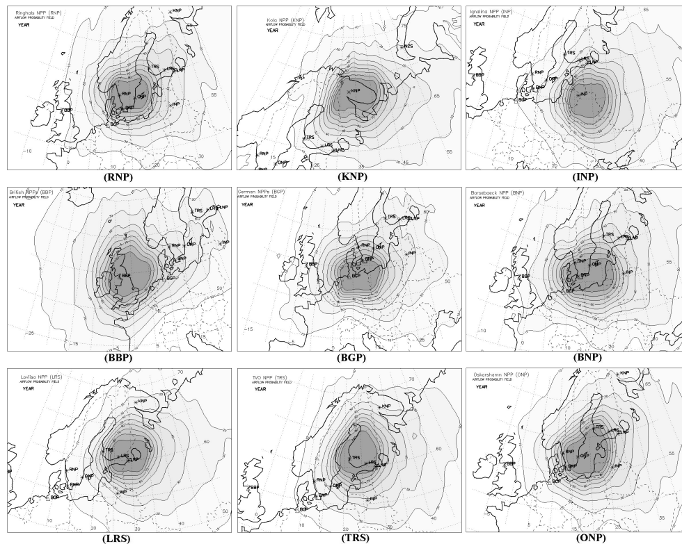
Fig. 3. Annual airflow probability fields for selected NRSs in the Euro-Arctic region.
