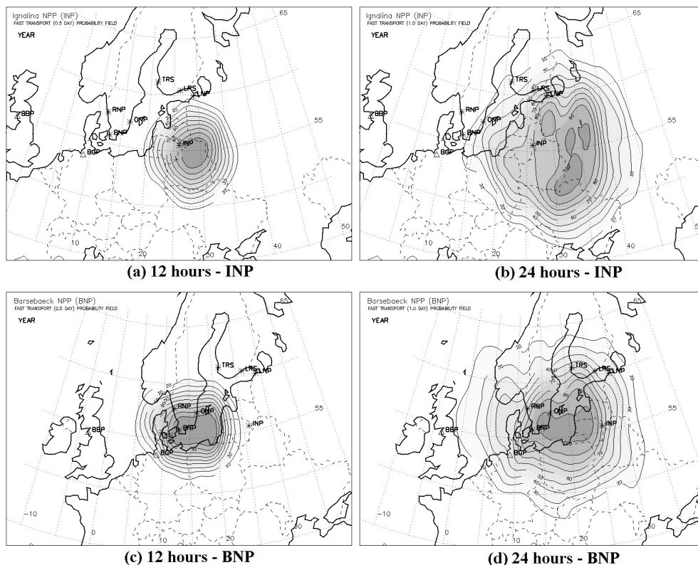
Fig. 8. Annual fast transport probability fields after 12 and 24 h of atmospheric transport from the Ilnalina NPP (INP) and Barsebaeck NPP (BNP).
