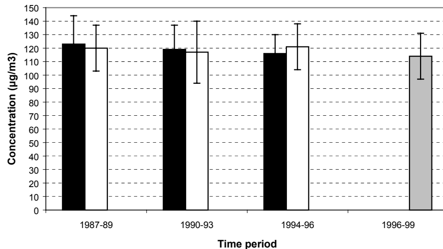
Fig. 11. Evolution of July–August rural afternoon (12:00–18:00) ozone levels at Aliartos (gray), Liossia (black) and Geoponiki (white) for 1987–1999 (only days with north winds and WS > 5 m/s were considered for the last two stations).
