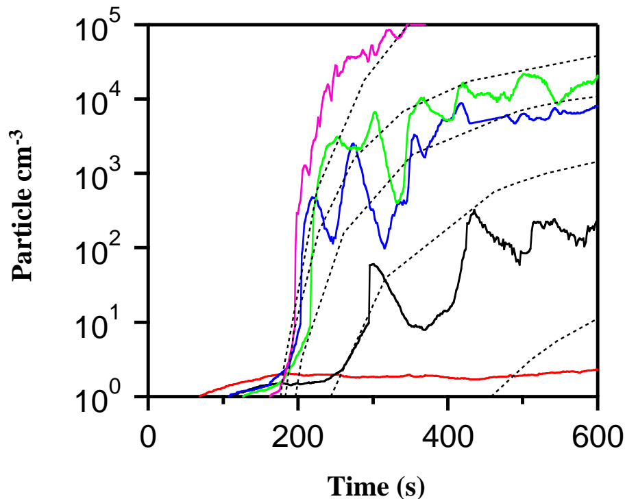
Fig. 8. Particle production following 30 s (red), 60 s (black), 90 s (blue), and 120 s (green) photolysis pulses (BLB365 lamps) with 185 ppt \text{CH}_2\text{I}_2 and 50 ppb \text{O}_3 . The particle production measured under these concentrations with continuous photolysis is shown for comparison (purple). The photolysis pulses correspond to I atom production concentrations of 6.8, 13.4, 19.7, and 25.8 ppt, respectively. The aerosol model simulations are given as the dashed lines (see text for details).
