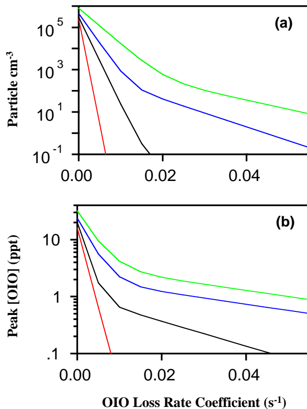
Fig. 11. Summary of atmospheric box-model calculations with T = 287\text{ K} and a diurnal IO profile with peak concentrations of 0.5 (red), 1.0 (black), 3.0 (blue), and 5.0 (green) ppt and a variable OIO first order loss rate coefficient (see text for details).
