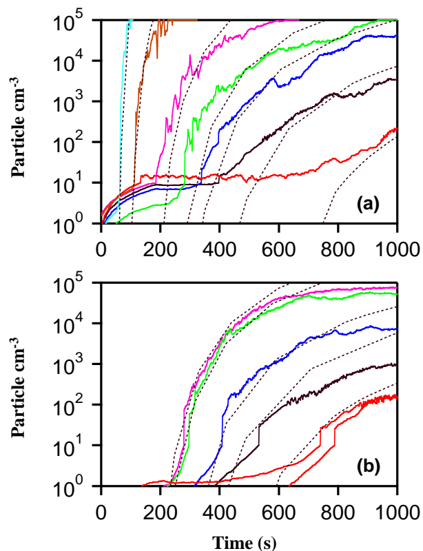
Fig. 7. Particle production dependence on the initial CH 2 I 2 concentration measured using BLB365 lamp continuous photolysis. (a) initial CH 2 I 2 concentrations of 0 (red), 15 (black), 29 (blue), 45 (green), 93 (purple), 531 (brown), and 1500 (light blue) ppt with 50 ppb O 3 . (b) initial CH 2 I 2 concentrations were 0 (red, two measurements), 6.6 (black), 13.7 (blue), 26.1 (green), and 41.4 (purple) ppt with 500 ppb O 3 . The aerosol model simulations are shown as dashed lines (see text for details).
