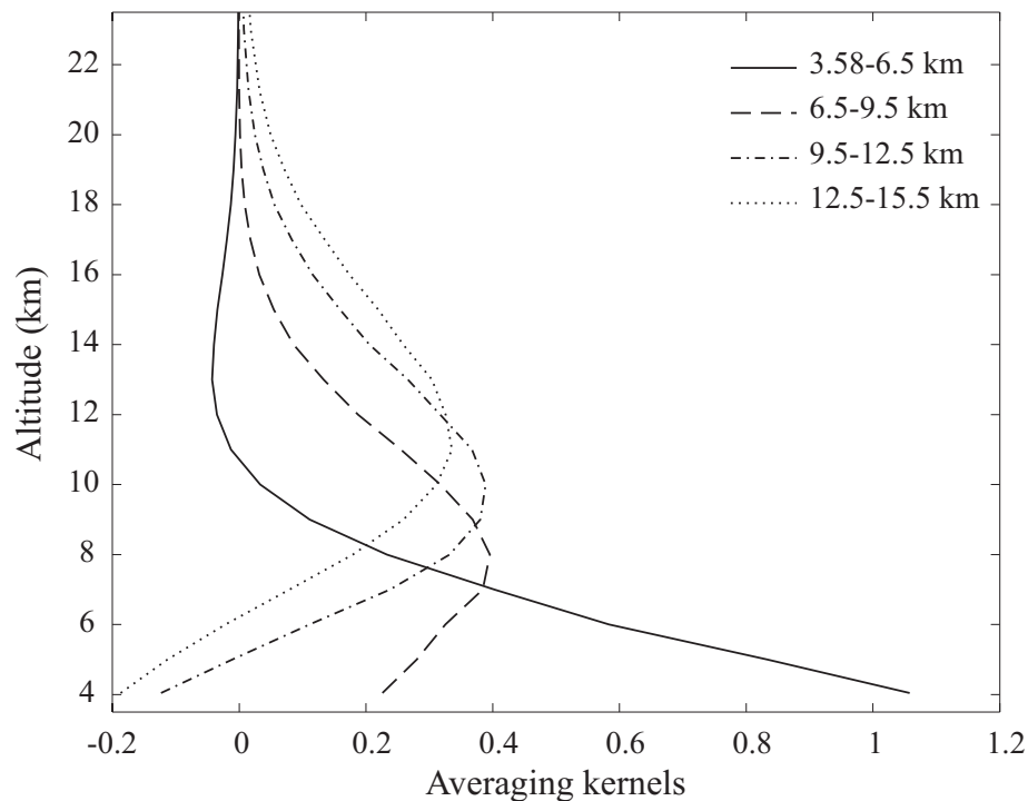
Fig. 1. CO vmr averaging kernels for 3 km thick merged layers from the ground up to 15.5 km. They have been calculated for a SZA (Solar Zenithal Angle) of 61^\circ and an OPD (Optical Path Difference) of 175 cm.
