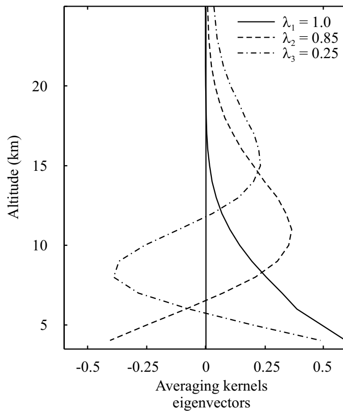
Fig. 2. Leading eigenvectors of the CO vmr averaging kernels (SZA=61°, OPD = 175 cm). The corresponding eigenvalues ( \lambda ) are given in the legend.
