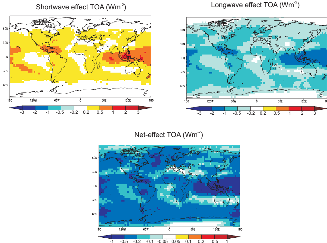
Fig. 6. Global shortwave, longwave and net TOA effect of cirrus clouds that have nucleated heterogeneously on solid OAD particles as compared to cirrus clouds formed in the absence of OAD. A positive shortwave effect means that less solar radiation is reflected to space. A negative longwave effect means that more longwave radiation is emitted to space.
