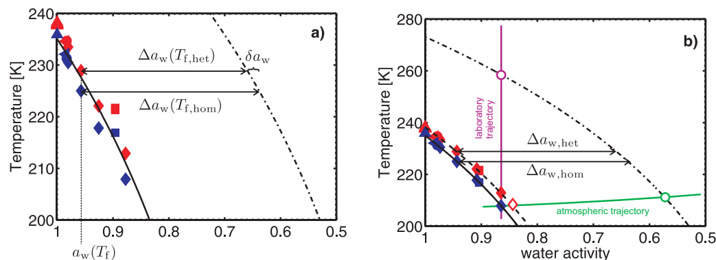
Fig. 2. Experimental freezing points of micrometer sized aqueous solution droplets. (a) Heterogeneous ice freezing points in the presence of OAD nano-crystals (red symbols) and homogeneous ice freezing points (reference, blue symbols) as a function of water activity. Upward triangles: water; left pointing triangles: SA/ABS; bullets: SA; diamonds: MA; squares: NaCl (see Table 2). Red and blue symbols appear as pairs at given water activity indicating the ice freezing temperatures of a specific solution in the presence or absence of OAD IN. The solid line is the homogeneous ice freezing curve for supercooled aqueous solutions and the dash-dotted line is the ice melting point curve (Koop et al., 2000). (b) Lines and symbols as in (a). The various pairs of freezing points were shifted horizontally such that the homogeneous freezing point of the reference sample is in accordance with the homogeneous freezing point line (solid). The magenta and green lines indicate a typical laboratory DSC trajectory and an atmospheric trajectory with ice melting points shown by the magenta and green circles, respectively. Under atmospheric conditions, aerosol particles containing OAD nano-crystals will nucleate ice heterogeneously at a lower water activity, and thus lower supersaturation (open red diamond) than is required for homogeneous ice nucleation without OAD (blue diamond).
