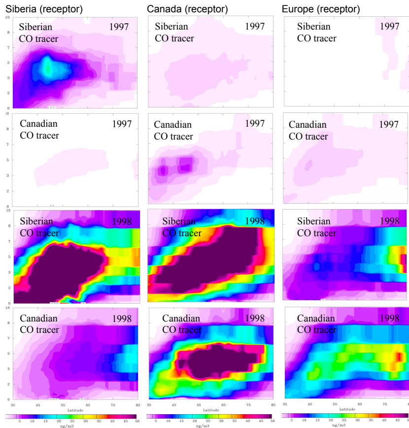
Fig. 4. Vertical cross sections of zonal means of the averaged CO tracer concentrations for the three receptor regions (see Fig. 3). Siberia (left column), Canada (middle column) and Europe (right column). The rows from top to bottom show the Siberian CO tracer in 1997, the Canadian CO tracer in 1997, the Siberian CO tracer in 1998 and the Canadian CO tracer in 1998 against altitude (km).
