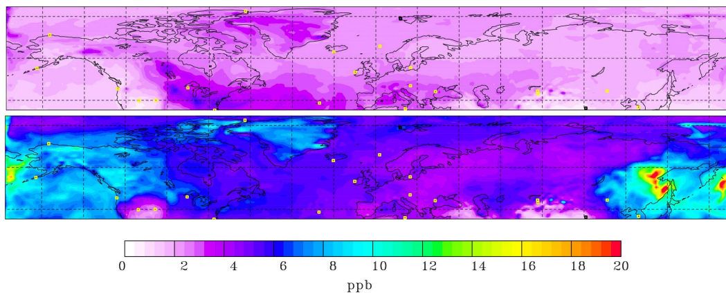
Fig. 5. FLEXPART mixing ratios at the lowest model layer in 1998; Canadian CO tracer (top), Siberian CO tracer (bottom); CMDL stations are marked as yellow squares.
