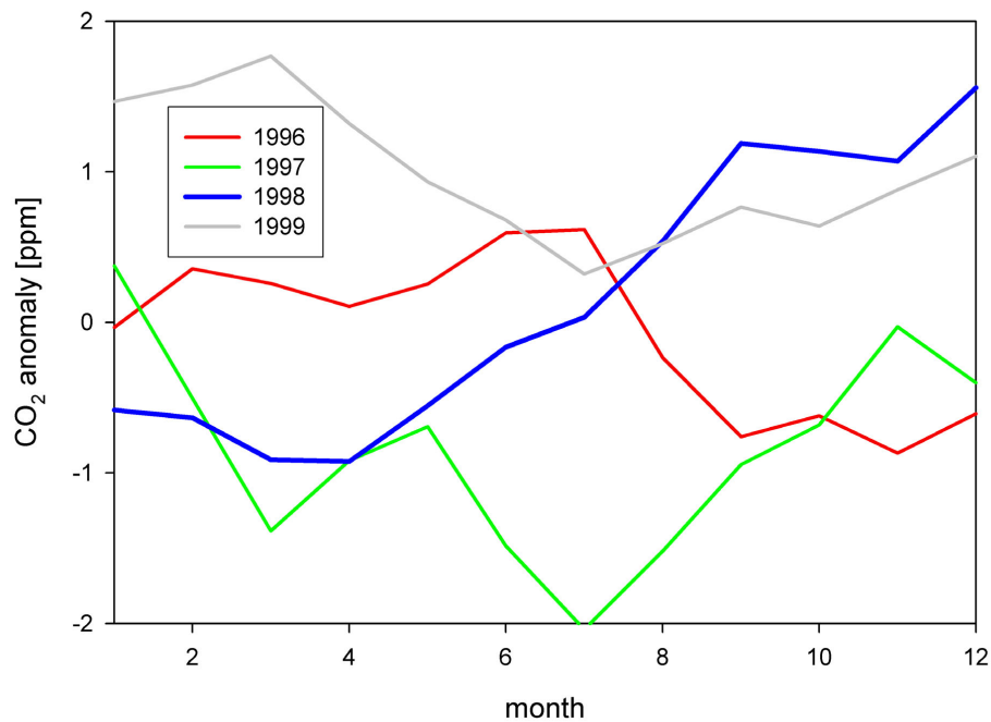
Fig. 6. Seasonal variation of the detrended anomalies (ppm) of CO 2 averaged over all CMDL stations north of 35° N.
