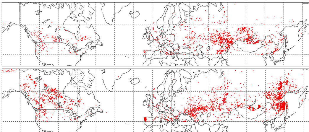
Fig. 2. ATSR hot spots summed from May to October of 1997 (top) and 1998 (bottom).
