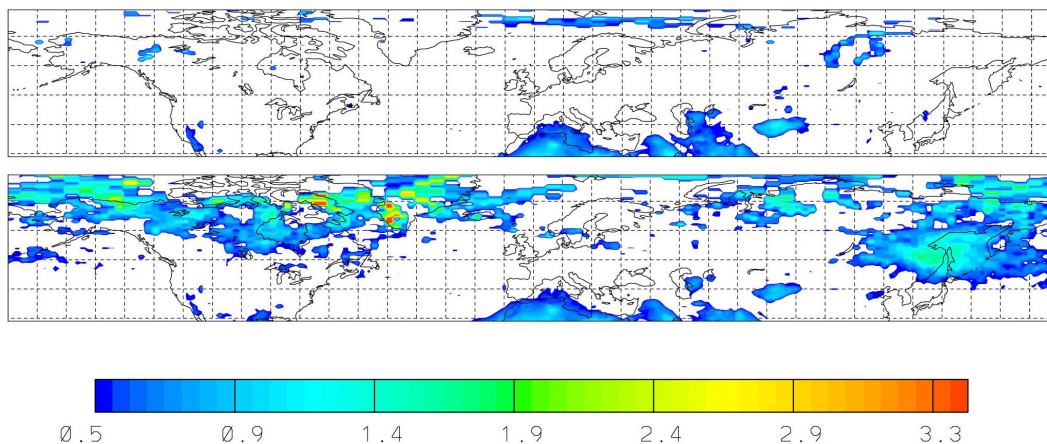
Fig. 9. TOMS aerosol index averaged from May to October 1997 (top) and 1998 (bottom).
