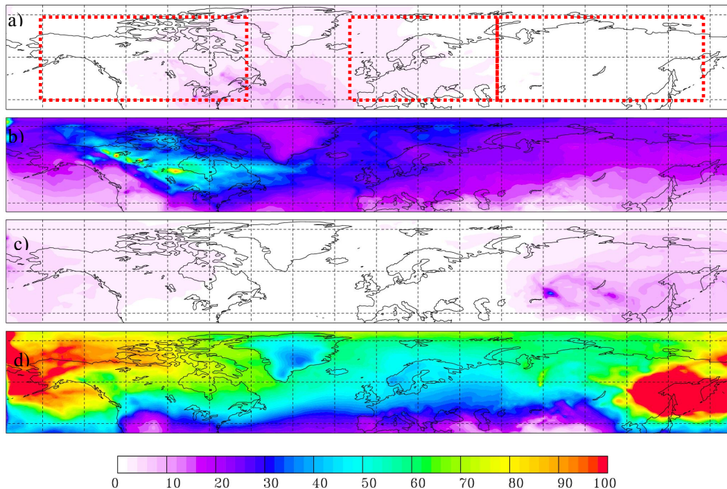
Fig. 3. Total columns of FLEXPART CO tracers ( \text{mg}/\text{m}^2 ) averaged from May to October: (a) Canadian CO tracer (1997), (b) Canadian CO tracer (1998), (c) Siberian CO tracer (1997) and (d) Siberian CO tracer (1998). The red boxes in panel (a) show the regions used for calculating source-receptor-relationships (see text for more details).
