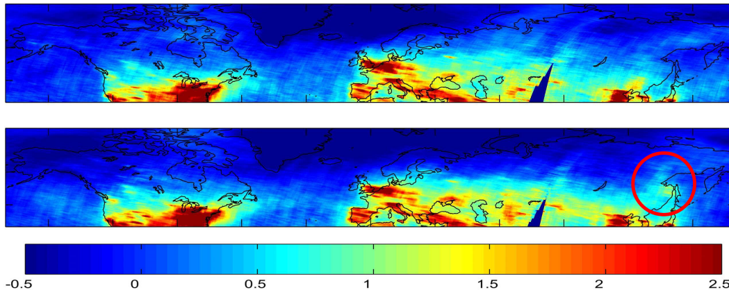
Fig. 10. GOME tropospheric \text{NO}_2 columns ( \text{molecules}/\text{cm}^2 ) averaged from July to August 1997 (top) and 1998 (bottom). The red circle marks enhanced \text{NO}_2 columns over eastern Siberia where the strongest fire activity occurred in 1998.
