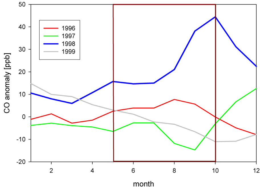
Fig. 7. Seasonal variation of the detrended anomalies (ppb) of CO averaged over all CMDL stations north of 35° N; the dark red rectangle reflects the burning season from May to October, which is shown in Fig. 8.
