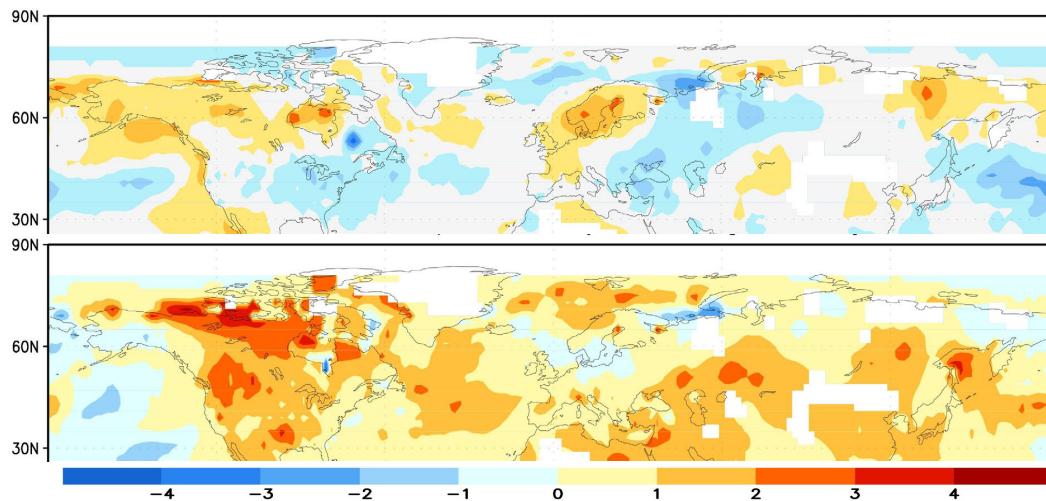
Fig. 1. Climatological surface temperature anomaly (K) from June to August of 1997 (top) and 1998 (bottom), according to NCEP reanalysis data.
