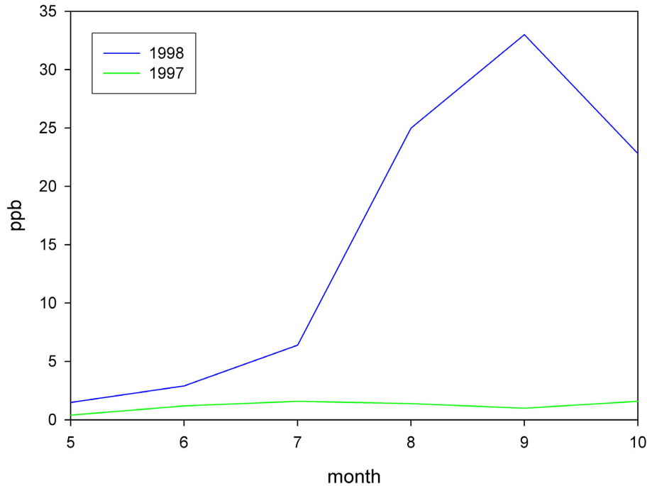
Fig. 8. Monthly mean FLEXPART CO tracer mixing ratios averaged for the positions of the CMDL stations.
