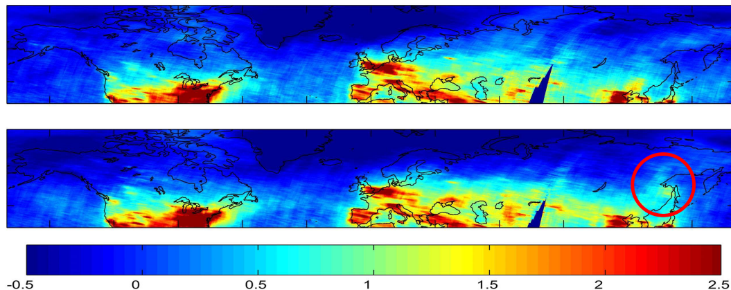
Fig. 10. GOME tropospheric \text{NO}_2 columns (molecules/ \text{cm}^2 ) averaged from July to August 1997 (top) and 1998 (bottom). The red circle marks enhanced \text{NO}_2 columns over eastern Siberia where the strongest fire activity occurred in 1998.
