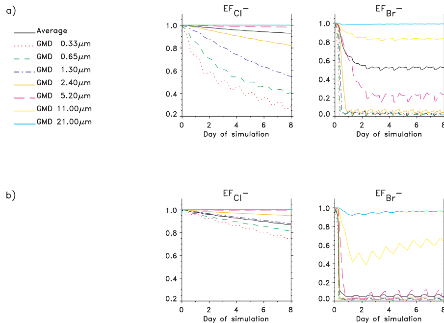
Fig. 6. Simulated concentrations of Cl^- and Br^- enrichment factors in sea-salt aerosols for model runs M1 (a) and M3 (b).
