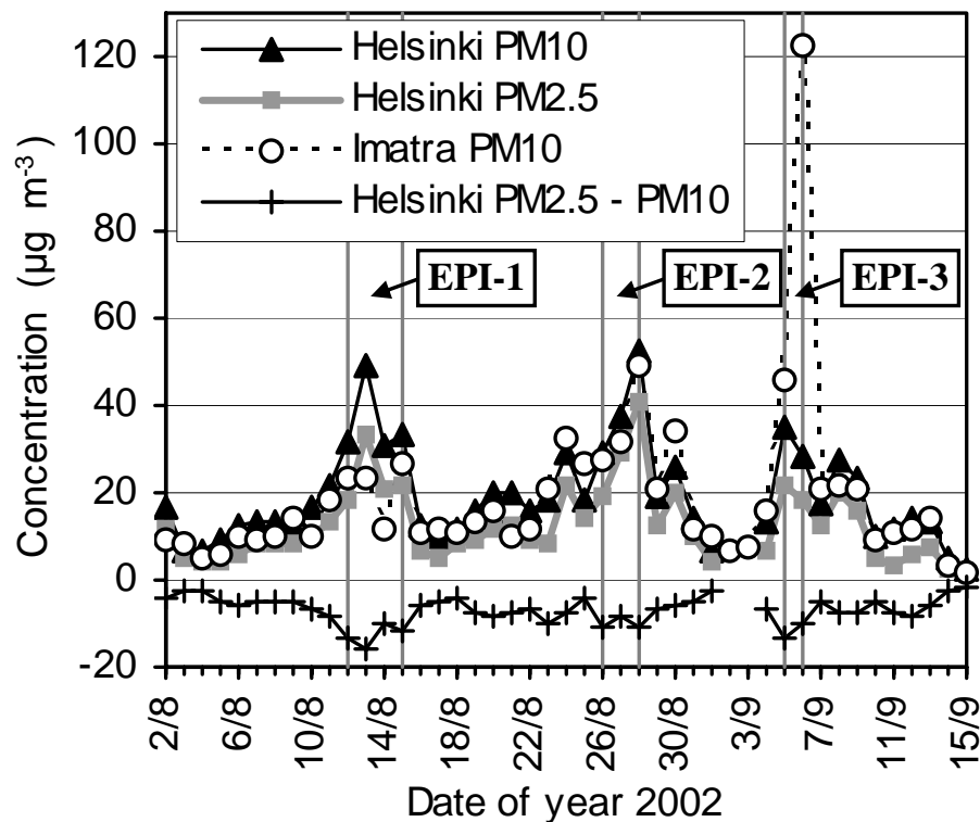
Fig. 2. Daily PM_{10} and PM_{2.5} concentrations at Kallio in Helsinki and daily PM_{10} concentration at Mansikkala in Imatra on 2 August–15 September 2002. The three strong LRT episode periods (EPI-1, EPI-2 and EPI-3) are marked out with vertical lines. Note that the concentrations of coarse particles are depicted for figure clarity as a subtraction PM_{2.5}-PM_{10} which gives negative values.
