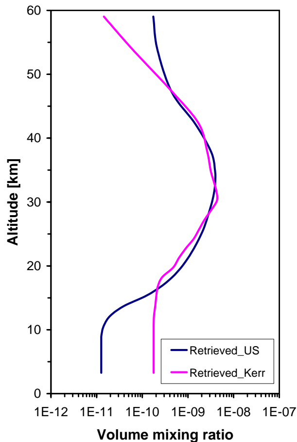
Fig. 1. NO 2 FTIR (profile scaling) retrieval results from one arbitrarily chosen measured spectrum with \text{SZA}=61^\circ using two different NO 2 a priori VMR profiles, i.e., the 1976 US Standard atmosphere (blue) versus the retrieval based upon the standard profile by “Kerr et al.” (Rinsland, personal communication, 1999), distributed with the “refmod99” data set (magenta).
