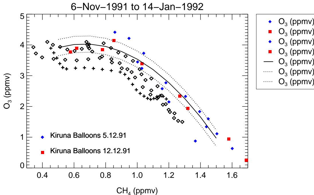
Fig. 2. The early winter reference function 1991–1992 shown as a black line was derived from balloon measurements from December 1991 (coloured symbols). Dotted lines indicate the range of uncertainty in the reference function. Observations made by HALOE within the vortex in November 1991 (black asterisks) and in January (black squares) are also shown.
