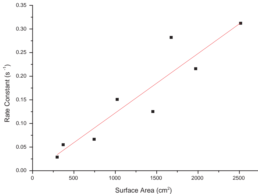
Fig. 5. Dependence of first-order rate constants for ozone loss as a function of film surface area ( [\text{O}_3]=1.4\text{--}3.0\times 10^{13} molecules \text{cm}^{-3} ).
