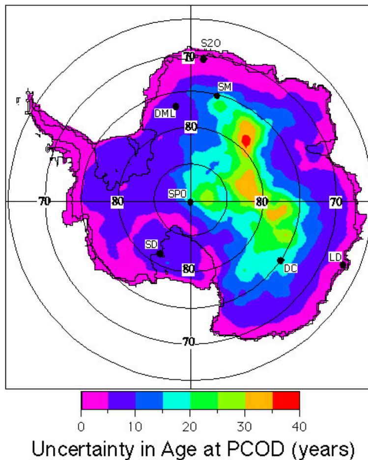
Fig. 12. The model uncertainty in derived \text{CO}_2 age at PCOD ( 2\sigma , in years). Here, twice the uncertainty ( 2\sigma ) for the tortuosity ( \gamma_b ) and the pore close-off density ( \rho_{\text{CO}} ) and a deviation of 5% in the modelled density profile were taken into account.
