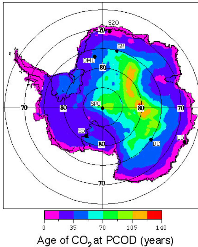
Fig. 10. The mean CO 2 age at PCOD in years, calculated with the pore close-off parameterisation of Martinerie et al. (1994) (Eq. 6a).
