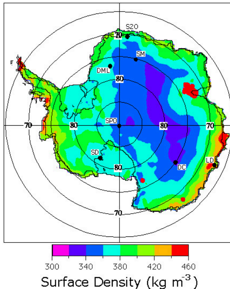
Fig. 5. The surface snow density field in \text{kg m}^{-3} , calculated using Eq. (5) in combination with Table 2.
