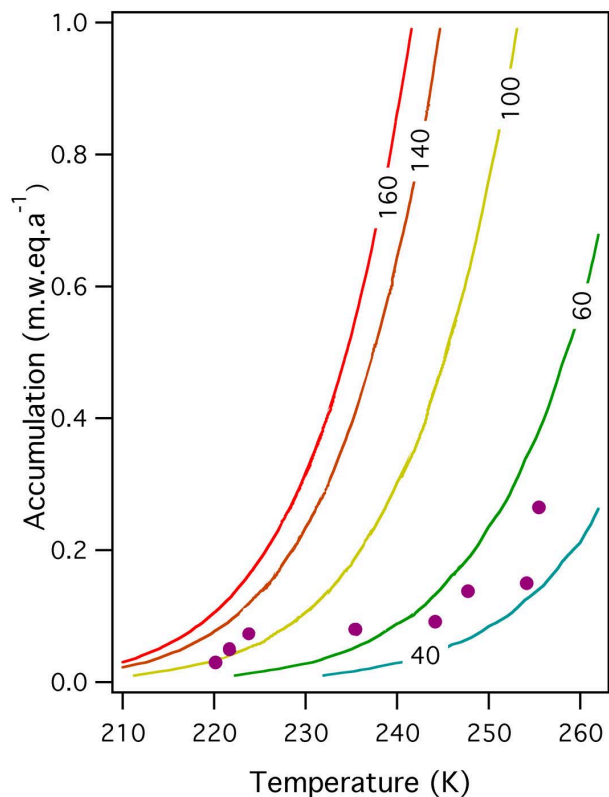
Fig. 7. Theoretically determined PCOD, using the density-depth model Herron and Langway (1980). The contour plot represents different PCOD's in m with varying annual surface temperatures and accumulation rates, varying from, respectively, 210 to 260 K and 0.01 to 1 m.w.eq.a -1 . The dots represent the PCOD's of nine sites (Table 1).
