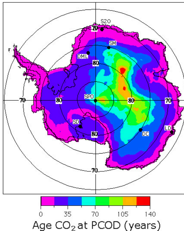
Fig. 9. The mean CO 2 age at PCOD in years for the entire Antarctic continent. The oldest CO 2 at PCOD, being 148 \pm 23 years ( 1\sigma ), is predicted as located at 43^\circ E and 78^\circ S.
