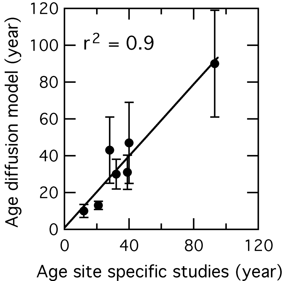
Fig. 4. Comparison between the modelled age of \text{CO}_2 at PCOD, using the parameterisations for \rho_0 , \rho_{\text{CO}} and \gamma_b (including the model uncertainty, 2\sigma ), and the obtained age of \text{CO}_2 at PCOD derived from site-specific studies (listed in Table 1).
