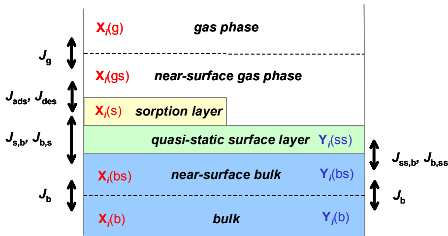
Fig. 2. Double-layer surface model compartments and transport fluxes for volatile species X_j (left) and non-volatile species Y_j (right).
