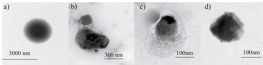
Fig. 3. TEM images of a) pure palmitic acid; b) and c) mixed ammonium sulfate/palmitic acid; and d) pure ammonium sulfate. Note the differences in the size bars.
