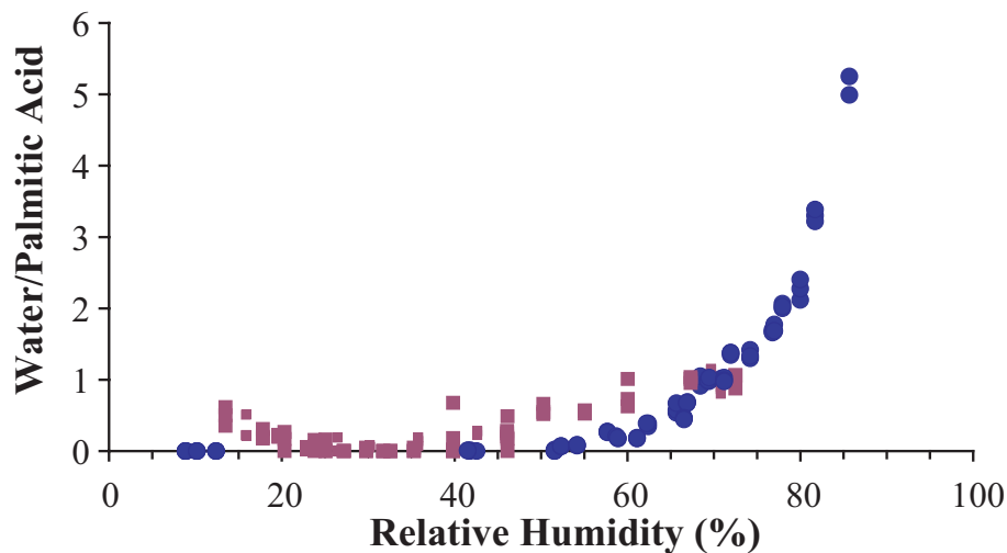
Fig. 7. Deliquescence (blue circles) and efflorescence (purple squares) of pure palmitic acid at 273 K.
