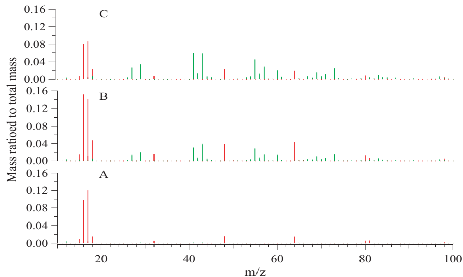
Fig. 4. AMS MS traces of ammonium sulfate/palmitic acid aerosol. The green indicate organic peaks and the red are sulfate peaks, A) pure ammonium sulfate; B) bath set to 120°C; and C) bath set to 140°C.
