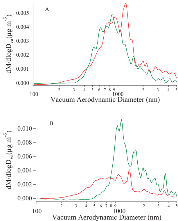
Fig. 5. TOF size distributions of A) palmitic acid bath at 120°C and B) bath at 140°C where the red is the ammonium sulfate trace and the green line is the organic trace.
