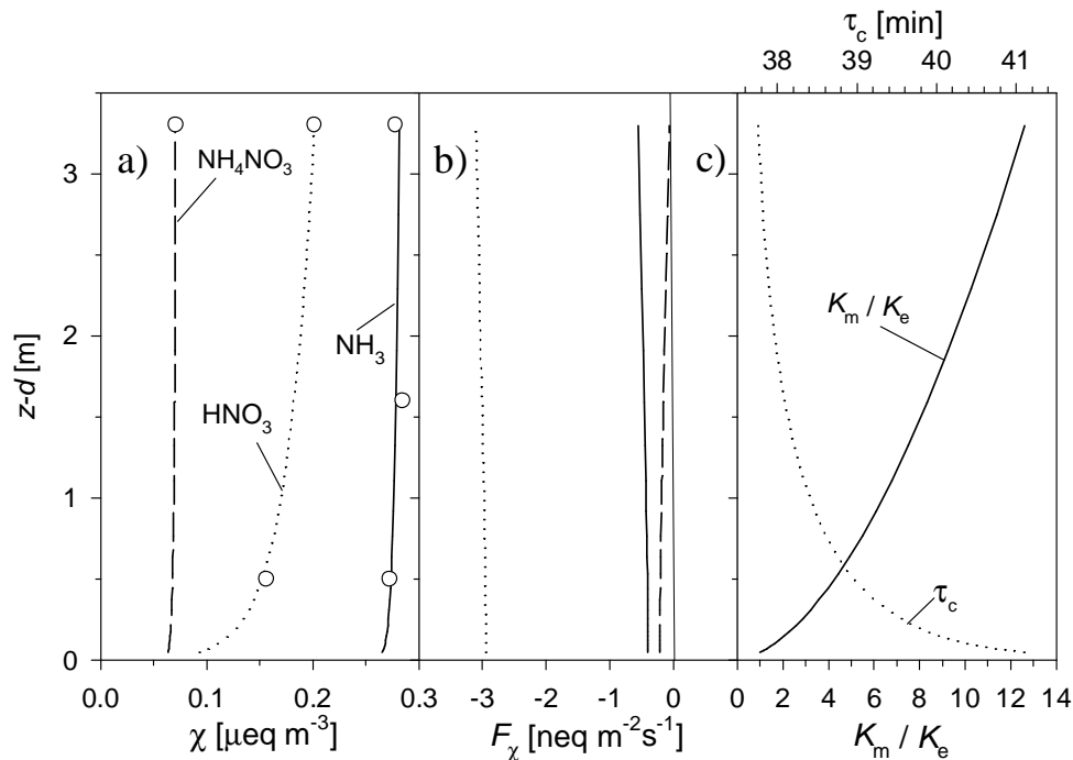
Fig. 8. Model output for 5 June 1996, 13:00 GMT using Scenario A. (a) Concentration gradients of the bulk species fitted to measured concentrations (O), (b) flux profiles and (c) height-dependence of the chemical time-scale ( \tau_c ) and the saturation ratio ( K_m/K_e ). The run uses \alpha=0.05 .
