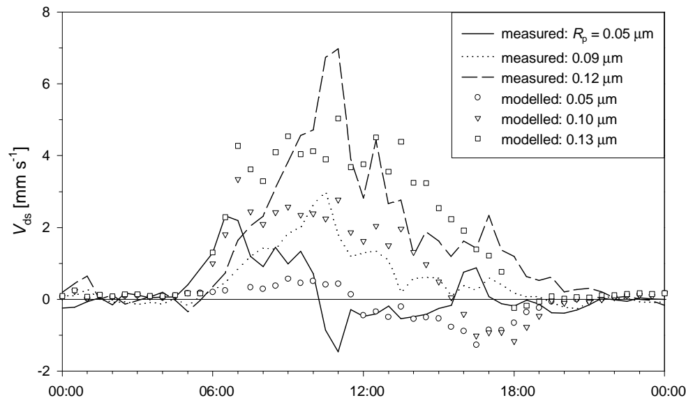
Fig. 13. Same as Fig. 10, but for Scenario D and \alpha=1 . V_{\text{ds}} is presented as derived from the fluxes at z_0 , as the model leads to small effects for the height of the ultrasonic anemometer (2.65 m), most likely due to an underestimation of z_{\text{eq}}=3.3 m (see text).
