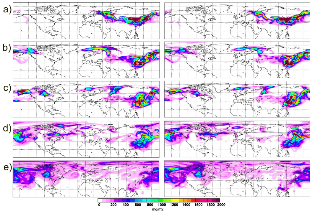
Fig. 2. Total CO tracer columns from simulations using ECMWF data (left column) and GFS data (right columns) on (a) 18 May 2003 at 00:00 UTC, (b) 21 May at 00:00 UTC, (c) 22 May at 06:00 UTC, (d) 26 May at 06:00 UTC and (e) 31 May at 00:00 UTC, respectively.
