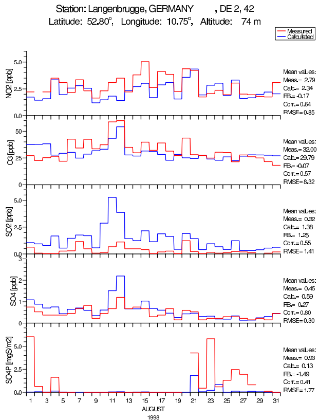
Fig. 14. Timeseries for the German station Langenbrügge for August 1998. Panels show from the top: atmospheric concentrations of NO 2 , O 3 , SO 2 , SO 4 2- and SO 4 2- in precipitation.
