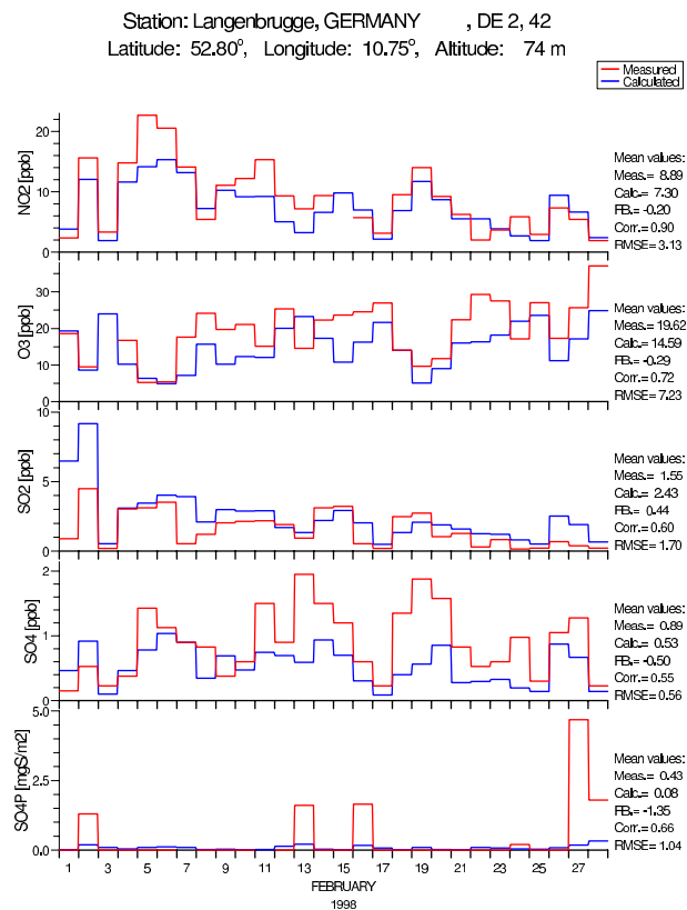
Fig. 8. Timeseries for the German station Langenbrügge for February 1998. Panels show from the top: atmospheric concentrations of \text{NO}_2 , \text{O}_3 , \text{SO}_2 , \text{SO}_4^{2-} and \text{SO}_4^{2-} in precipitation.
