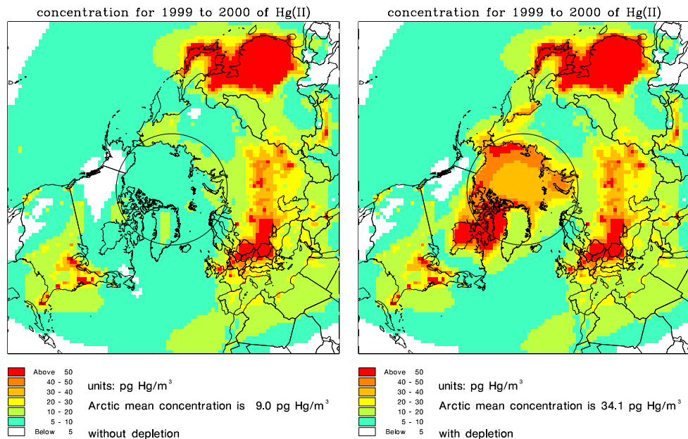
Fig. 4. The concentration of RGM (=Hg(II)) in \text{pg Hg/m}^3 ; without the fast oxidation rate causing Arctic mercury depletion (left) and with the fast oxidation rate (right).
