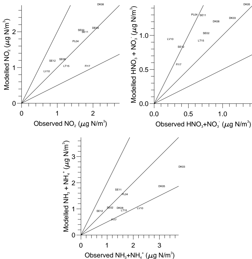
Fig. 1. Comparison between observed and calculated nitrogen dioxide, the sum of nitric acid and aerosol phase nitrate, and NH x (the sum of NH 3 and NH 4 + ) at the 16 selected stations in the EMEP programme. Annual mean values for 1999. The stations in the figure is explained in Appendix 1 and strait lines indicate 1:1, 1:2 and 2:1, respectively.
