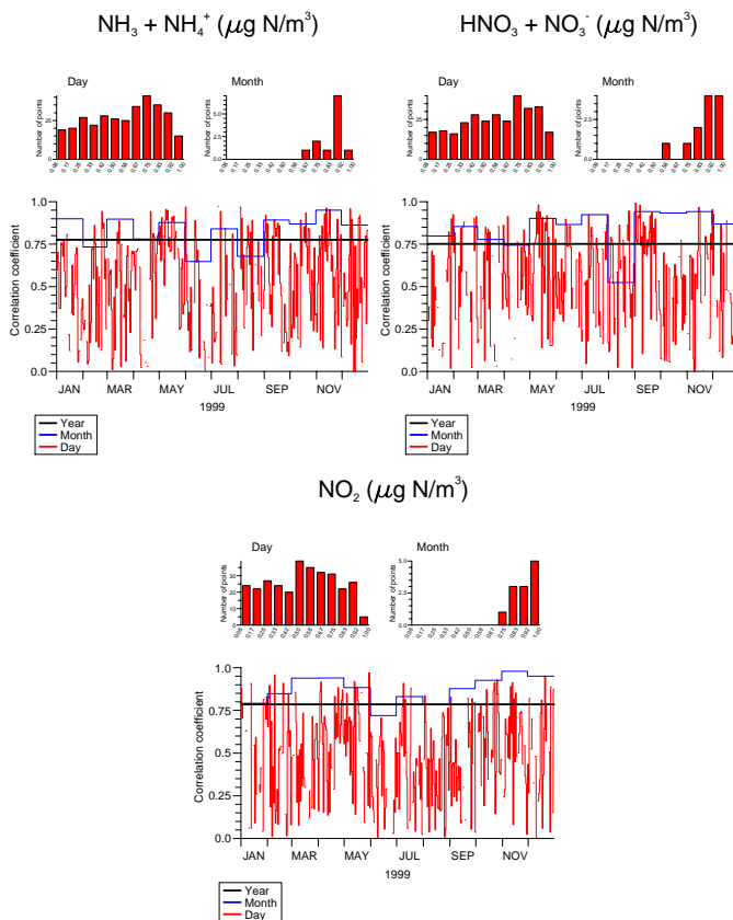
Fig. 6. Correlation coefficients between observed and modelled \text{NH}_x (sum of \text{NH}_3 and \text{NH}_4^+ ), total nitrate (sum of \text{HNO}_3 and \text{NO}_3^- ) and \text{NO}_2 for annual, monthly and diurnal mean values – all data for the year 1999. The averaging is performed over the 16 selected EMEP stations for each set of data.
