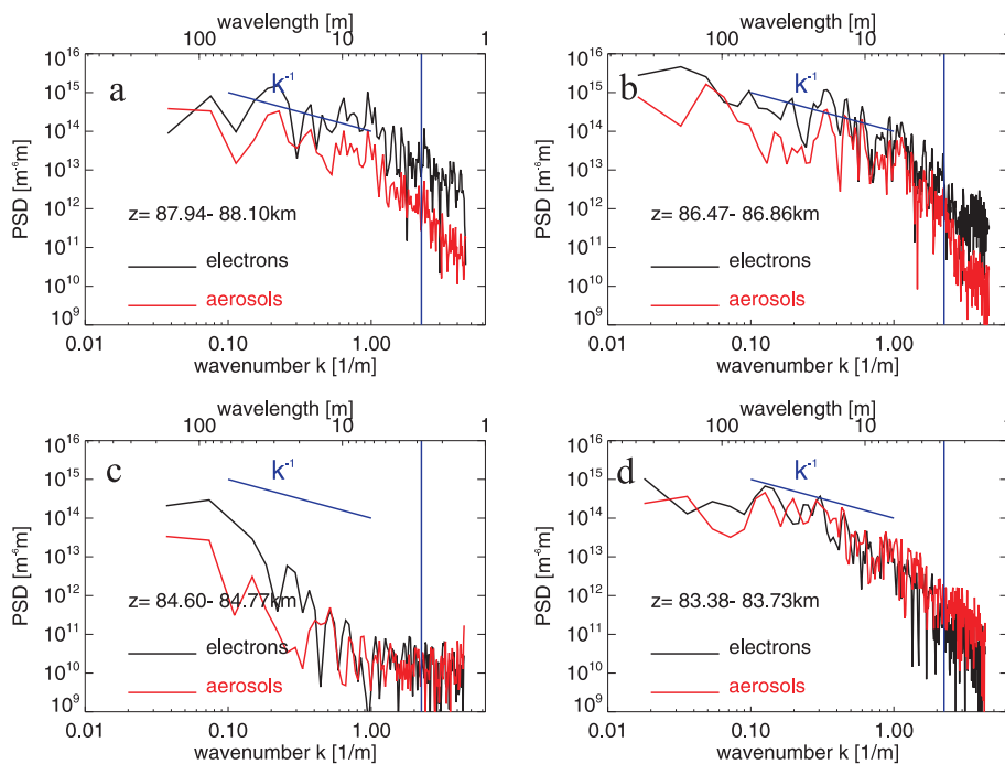
Fig. 7. Power spectra of electron number density (black lines) and particle charge number density fluctuations (red lines) shown in the Figs. 3 and 4, respectively. Note that principally the data presented have been measured in the time rather than in the spatial domain. Wavenumbers have been determined from measured frequencies f applying the relation k = 2\pi f/v_R where v_R is the rocket velocity ( \sim 800 m/s in our cases). The inclined line represents a spectral slope of -1 and the vertical line marks the radar Bragg scale ( =2.8 m).
