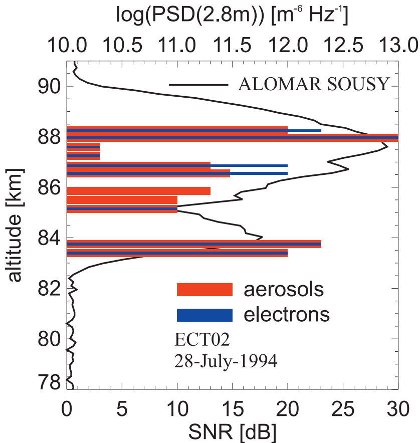
Fig. 5. Comparison of the radar signal to noise ratio, SNR, during the sounding rocket flight ECT02 (black line, lower abscissa) and N_e^2 \cdot \text{PSD}(\frac{\Delta N_e}{N_e}, \lambda/2) as well as N_A^2 \cdot \text{PSD}(\frac{\Delta N_A}{N_A}, \lambda/2) (red bars for charged aerosol particles, blue bars for electrons, upper abscissa).
