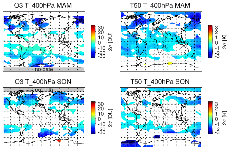
Fig. 3. Size of fluctuations attributed to temperature anomalies at 400 hPa. The size is defined as 2 standard deviations, in DU or K, of the c_{T(400)} T(400) time series term in Eq. (1). In this plot and the following, blue colors (negative values) indicate that ozone or temperature are inversely (negatively) correlated to the explanatory variable, whereas yellow and red colors (positive values) denote positive correlation. In the white regions the explanatory variable is not statistically significant at the 90% confidence level. Also note that no TOMS/SBUV observations are available in polar regions in winter.
