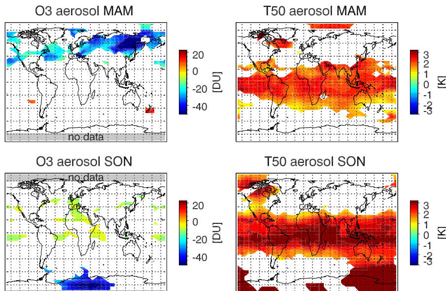
Fig. 8. Same as previous figures, but showing the ozone and 50 hPa temperature response to stratospheric aerosol from the El Chichón and Pinatubo eruption. Here the maximum positive or negative response is shown, not two standard deviations as in the other plots.
