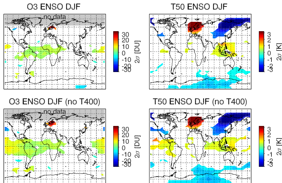
Fig. 11. Same as previous Figures, but showing the influence of El Niño/Southern-Oscillation on total ozone and 50 hPa temperature. Top panels: Obtained with full set of explanatory variables, including 400 hPa temperature. Bottom panels: Reduced set of explanatory variables, without 400 hPa temperature.
