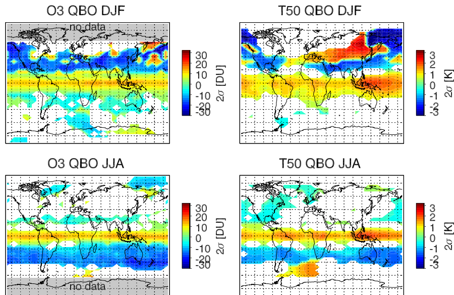
Fig. 4. Same as Fig. 3 but for fluctuations attributed to the QBO ( 2\sigma of term c_{QBO(10)} QBO(10) + c_{QBO(30)} QBO(30) in Eq. (1)). Here, blue colors indicate inverse (negative) correlation with westerly zonal wind at 30 hPa at the Equator, whereas yellow and red colors indicate positive correlation.
