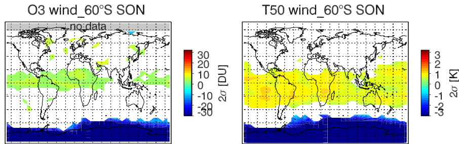
Fig. 10. Same as Fig. 9, but for zonal wind anomalies at 60° S, 50 hPa.
