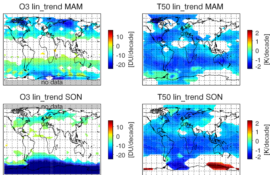
Fig. 2. Left panels: Linear trend, in DU per decade, from multiple regression of 1978 to 2001 TOMS/SBUV total ozone anomalies on a 5° latitude by 10° longitude grid. Right panels: Linear trend, in K per decade, from multiple regression of 1978 to 2001 temperature anomalies at 50 hPa from NCEP reanalyses on a 5° latitude by 10° longitude grid. In the white regions the linear trend is not statistically significant at the 90% confidence level. Also note that no TOMS/SBUV observations are available in polar regions in winter.
