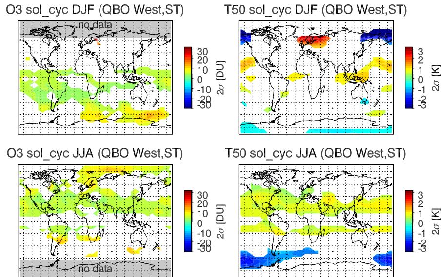
Fig. 7. Same as Fig. 6 but for the westerly phase of the QBO (at 50 hPa). To improve clarity for this figure, as well as for Fig. 6, the confidence level was reduced to 80%, and zonal winds at 60° N and 60° S were not included as explanatory variables.
