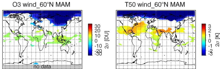
Fig. 9. Same as previous figures, but showing the influence of polar vortex strength, represented by zonal wind anomalies at 60° N, 50 hPa, on total ozone and 50 hPa temperature.
