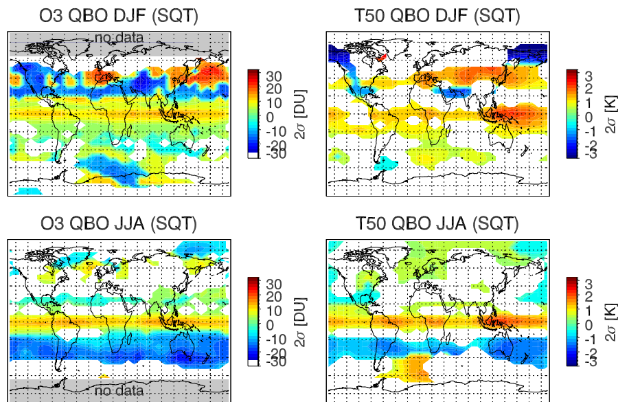
Fig. 5. Same as Fig. 4 but for regression with a reduced set of explanatory variables, containing only QBO, solar cycle and a linear trend.
