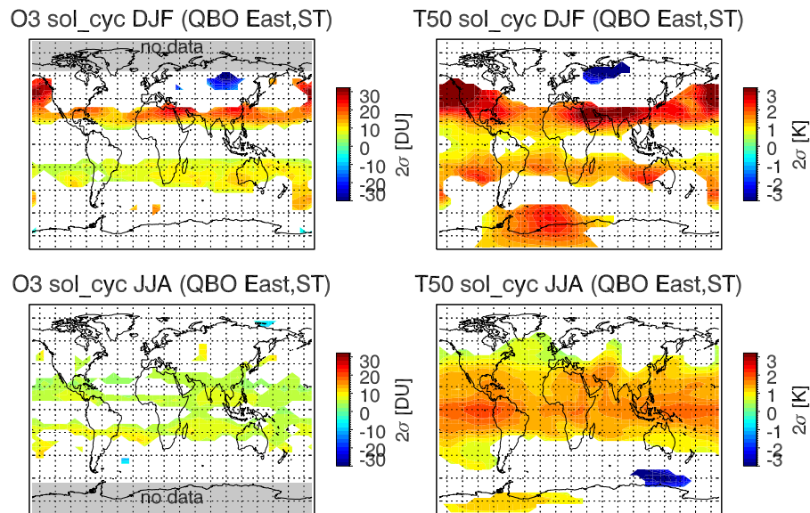
Fig. 6. Same as Fig. 4 but for total ozone fluctuations associated with the 11-year solar cycle. Yellow and red colors indicate positive correlation between total ozone and solar flux. Only data during the easterly phase of the QBO (at 50 hPa) are used. To improve clarity for this figure, as well as for Fig. 7, the confidence level was reduced to 80%, and zonal winds at 60° N and 60° S were not included as explanatory variables.
