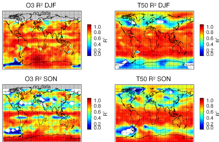
Fig. 1. Global maps of R^2 from regression of 1978 to 2001 TOMS/SBUV total ozone anomalies on a 5^\circ latitude by 10^\circ longitude grid (left panels), or of 1978 to 2001 50 hPa temperature anomalies from NCEP reanalyses (right panels). No TOMS/SBUV observations are available in polar regions in winter.
