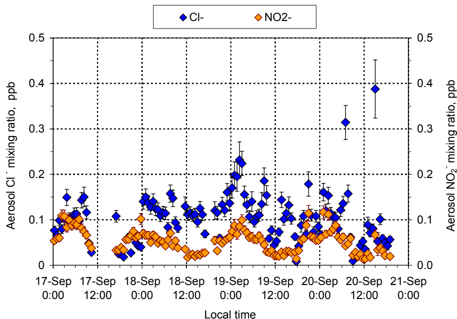
Fig. 10. Diel variations of aerosol \text{Cl}^- and \text{NO}_2^- (fine fraction, <2.5 \mu\text{m} ) during 17 to 20 September 2002 (biomass burning season) at FNS. Error bars indicate measurement uncertainty for each data point.
